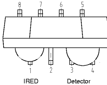
Figure 2. Pinning
