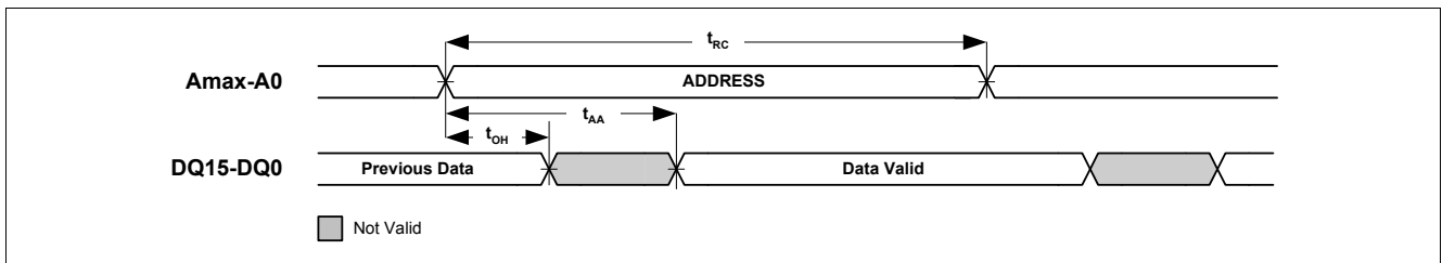
Figure 20 Asynchronous Read - Address Controlled ( \overline{CS} = \overline{OE} = V_{IL} , \overline{WE} = V_{IH} , \overline{UB} and/or \overline{LB} = V_{IL} , \overline{CRE} = V_{IL} , \overline{ADV} = V_{IL} )
