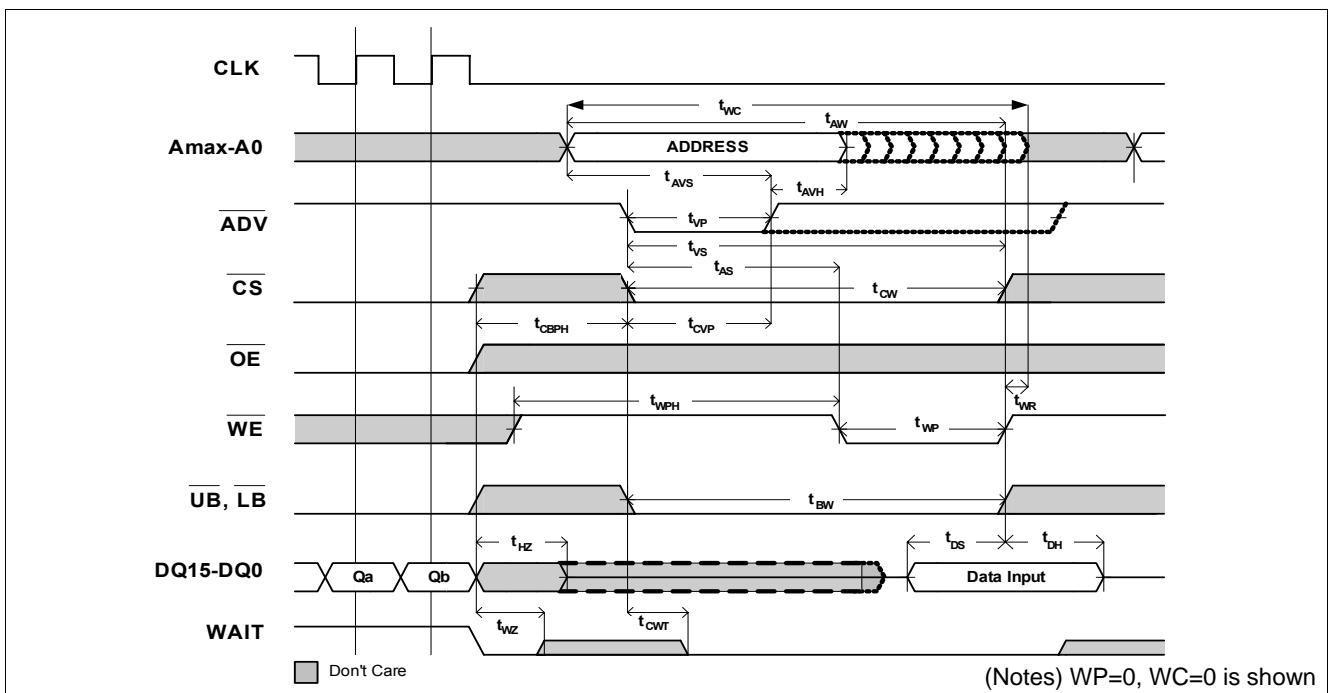
Figure 32 Asynchronous Write with Address Latch ( \overline{ADV} ) Control
