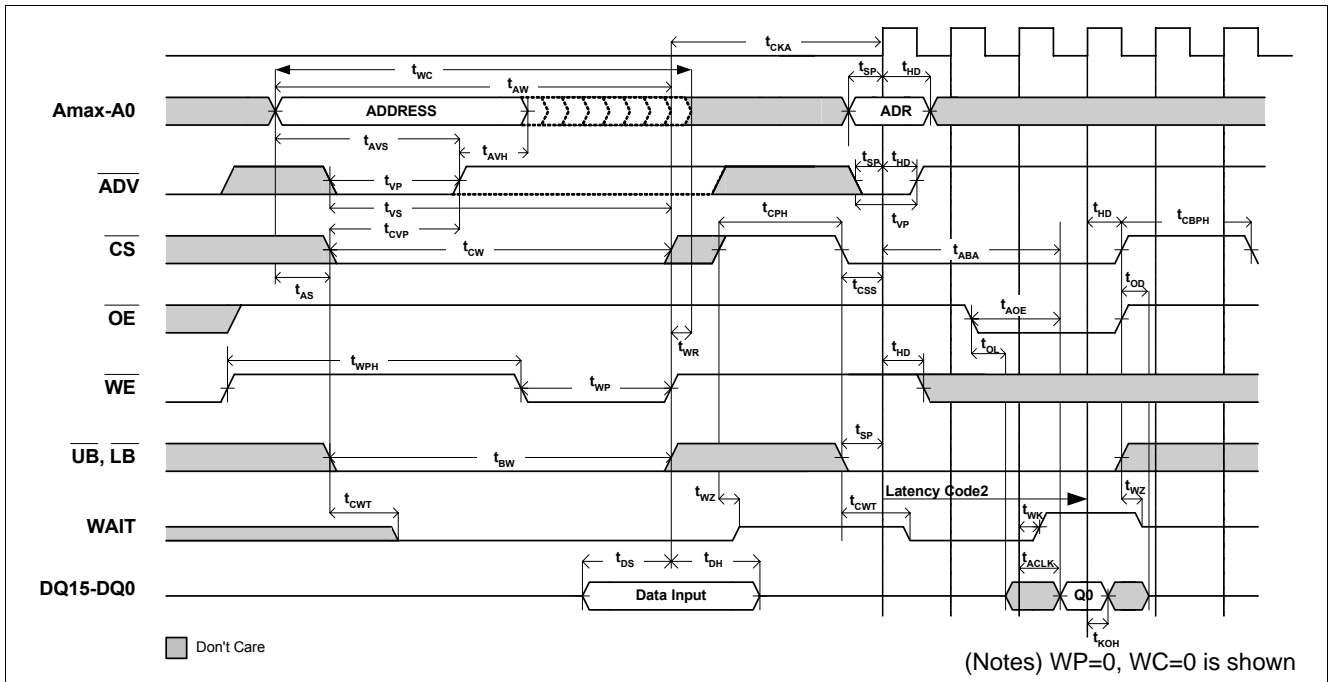
Figure 31 Asynchronous Write with Address Latch ( \overline{ADV} ) Control (followed by single-burst read)
