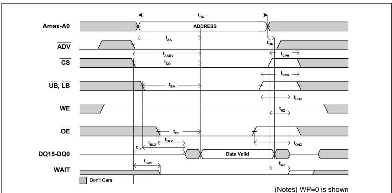
Figure 21 Asynchronous Read ( \overline{WE} = V_{IH} , \overline{CRE} = V_{IL} )
