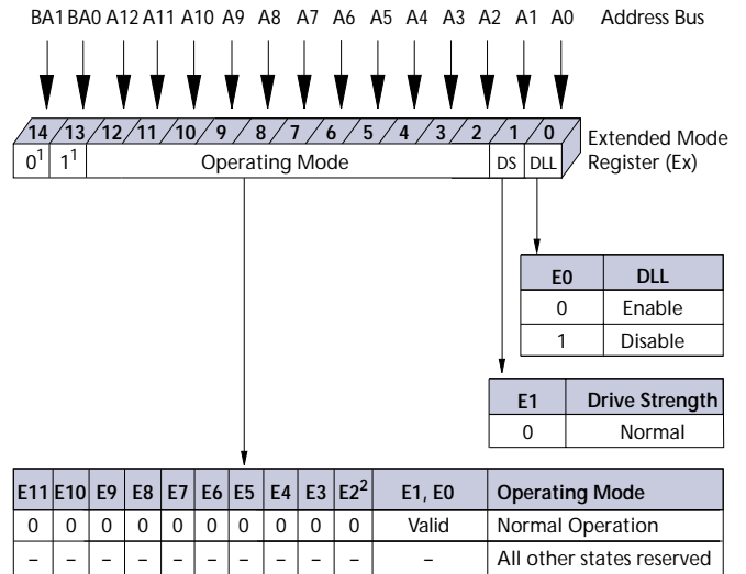
Figure 6: Extended Mode Register Definition Diagram
