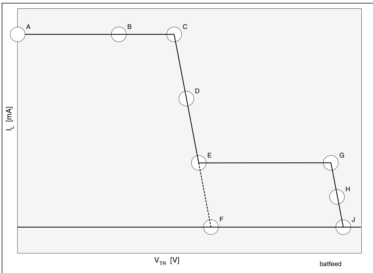
Figure 12 Battery Feed Characteristics
