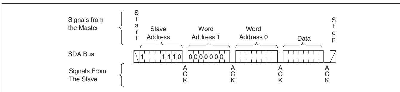
Figure 13. Writing 30 bytes to a 64-byte memory page starting at address 40.
