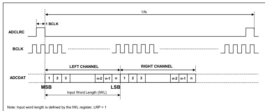
Figure 16 DSP Mode
