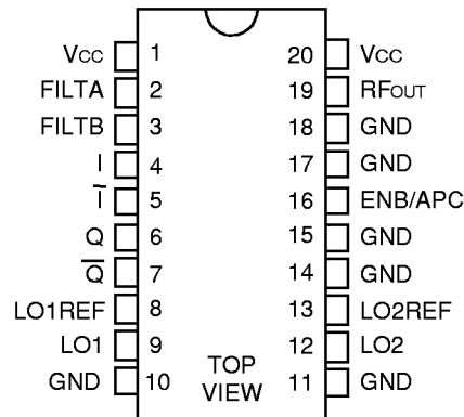
Figure 2. Pin Diagram
