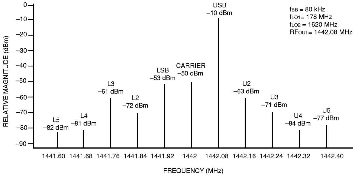
Figure 3. W3013 Sine-Wave Modulation Output Spectrum
