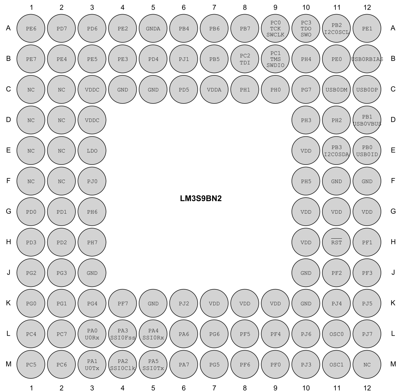
Figure 23-2. 108-Ball BGA Package Pin Diagram (Top View)
