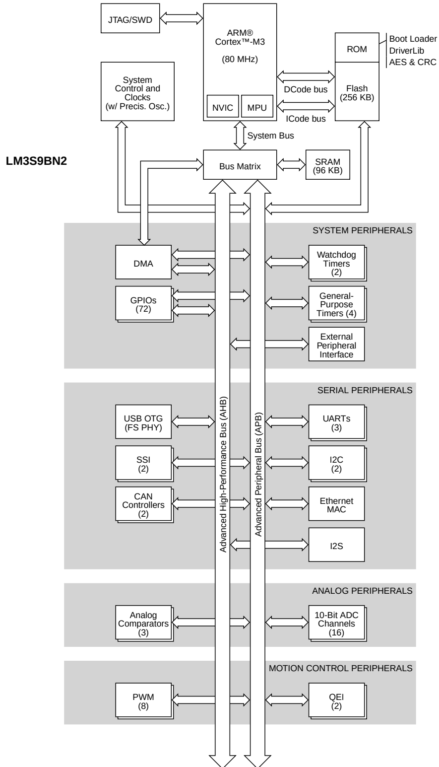
Figure 1-1. Stellaris LM3S9BN2 Microcontroller High-Level Block Diagram
