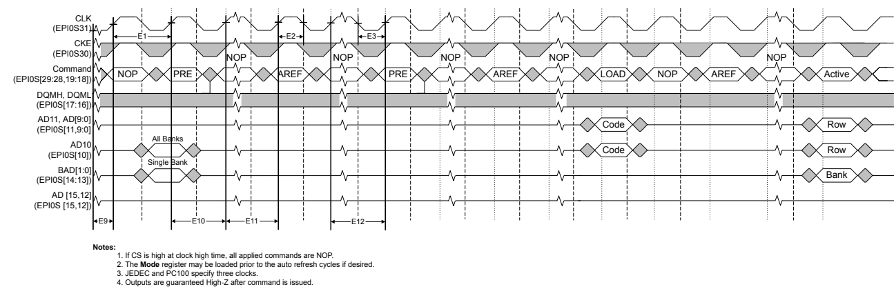
Figure 26-11. SDRAM Initialization and Load Mode Register Timing
