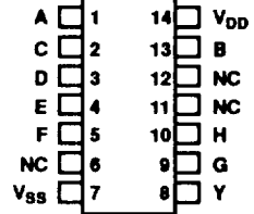
14-Pin DIP Top View
