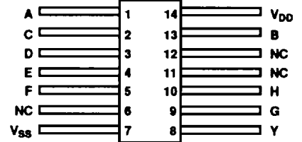
14-Lead Flatpack Top View
