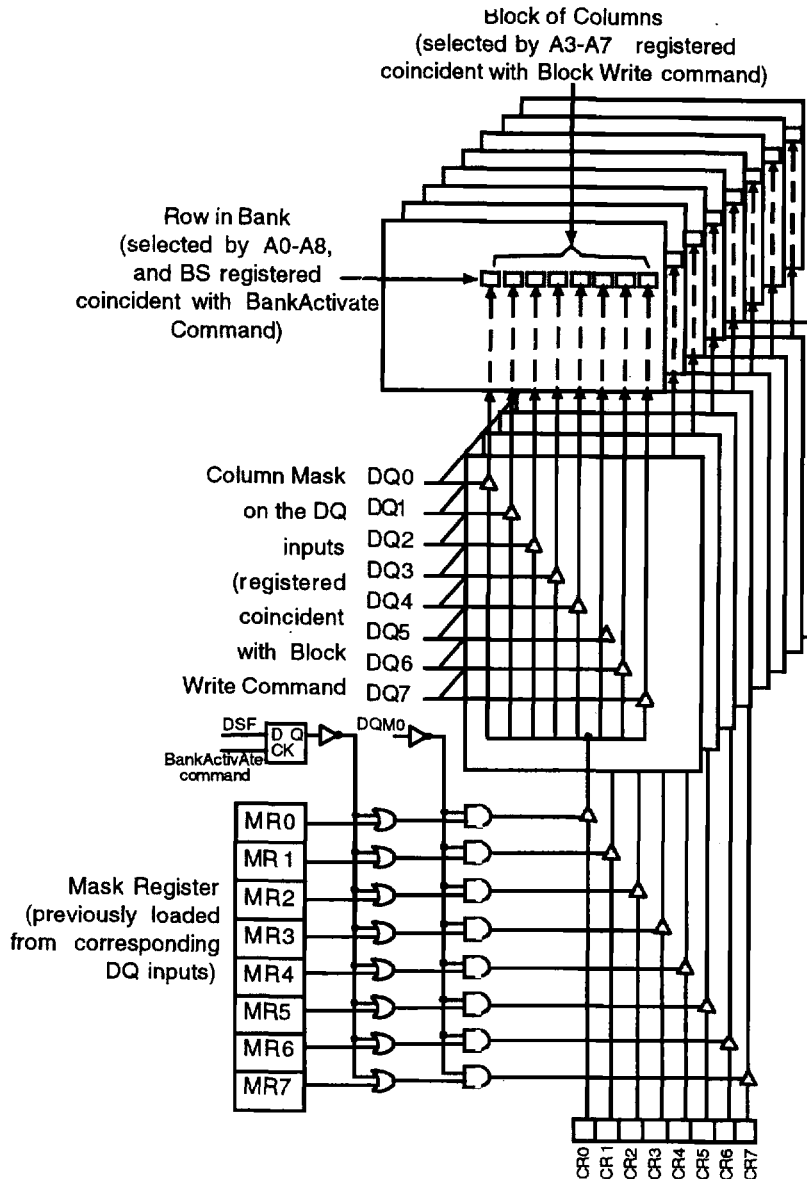
Block-Write Masking Block Diagram
