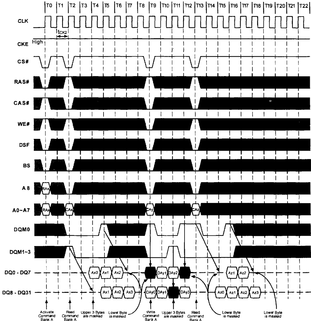
Figure 20. Byte Write Operation (Burst Length=4, CAS# Latency=2)
