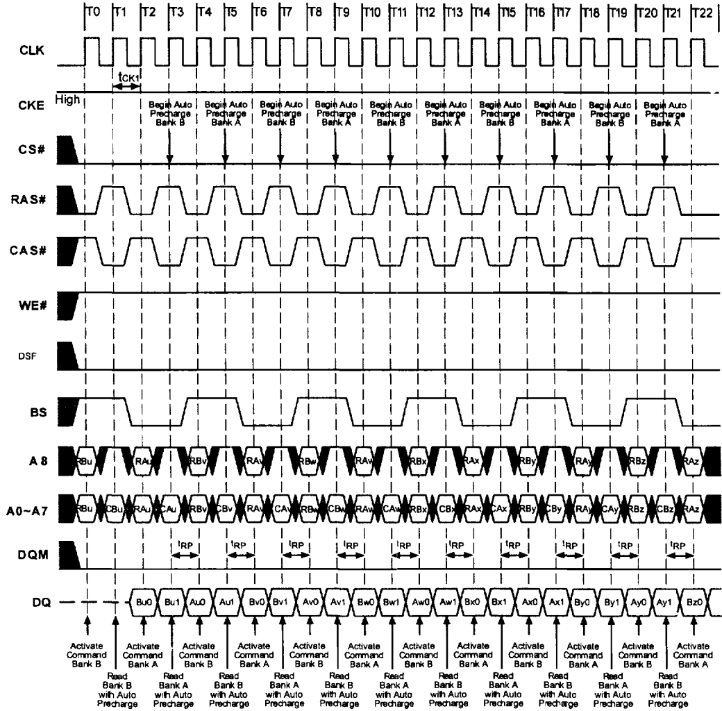
Figure 23. Random Row Read (Interleaving Banks)
