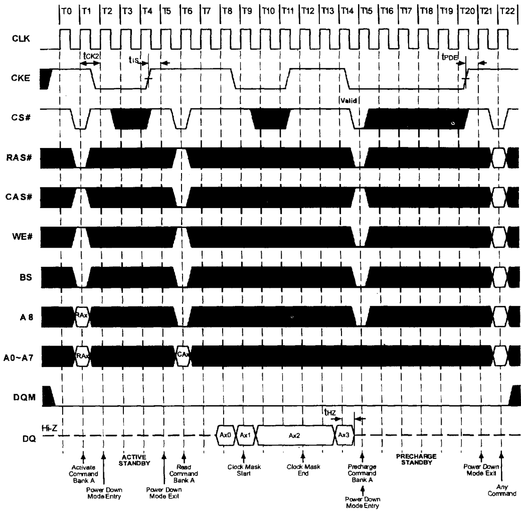
Figure 8. Power Down Mode and Clock Mask (Burst Length=4, CAS# Burst Length=4, CAS# Latency=2)
