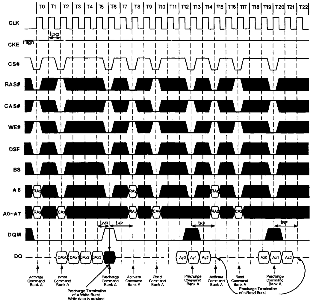
Figure 26.2. Precharge Termination of a Burst (Burst Length=8 or Full Page, CAS# Latency=2)
