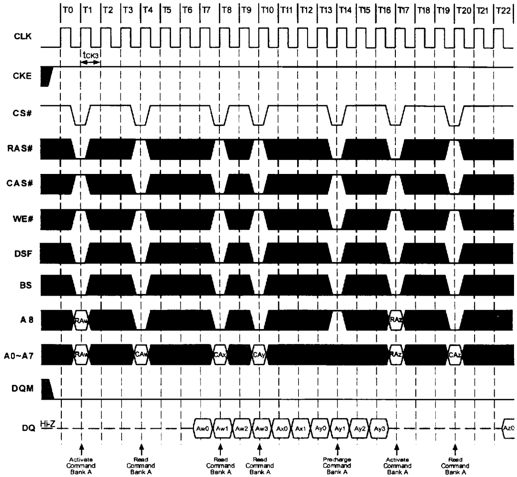
Figure 9.3. Random Column Read (Page within same Bank) (Burst Length=4, CAS# Latency=3)
