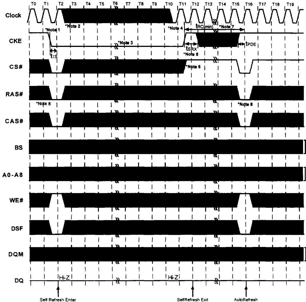
Figure 5. Self Refresh Entry & Exit Cycle
