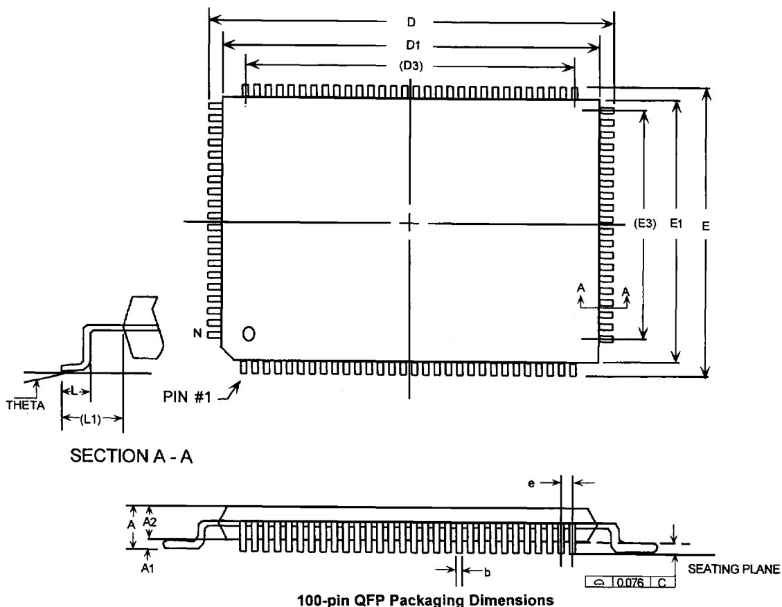
100-pin QFP Packaging Dimensions
