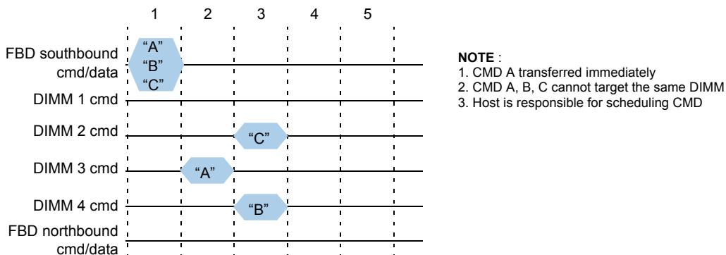
Figure 6. FBDIMM Command Delivery Rules
