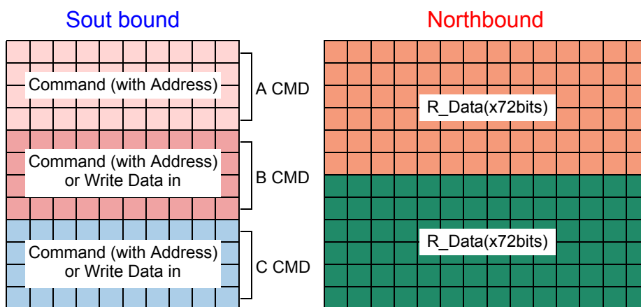
Figure 4. Southbound / Northbound Frame format
