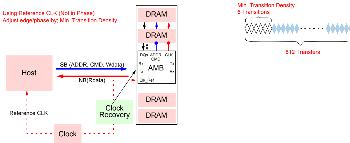
Figure 3. FB-DIMM Clocking
