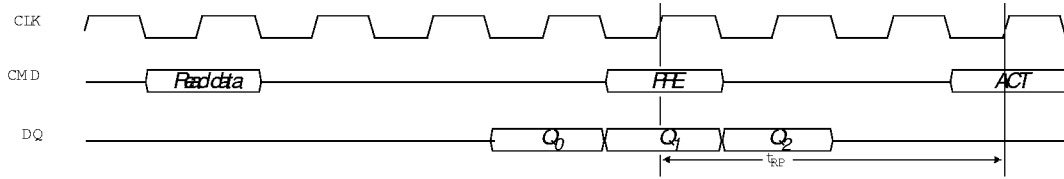
read cycle (CL = 3)
