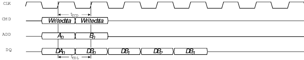
write interrupted by write (BL = 4)
