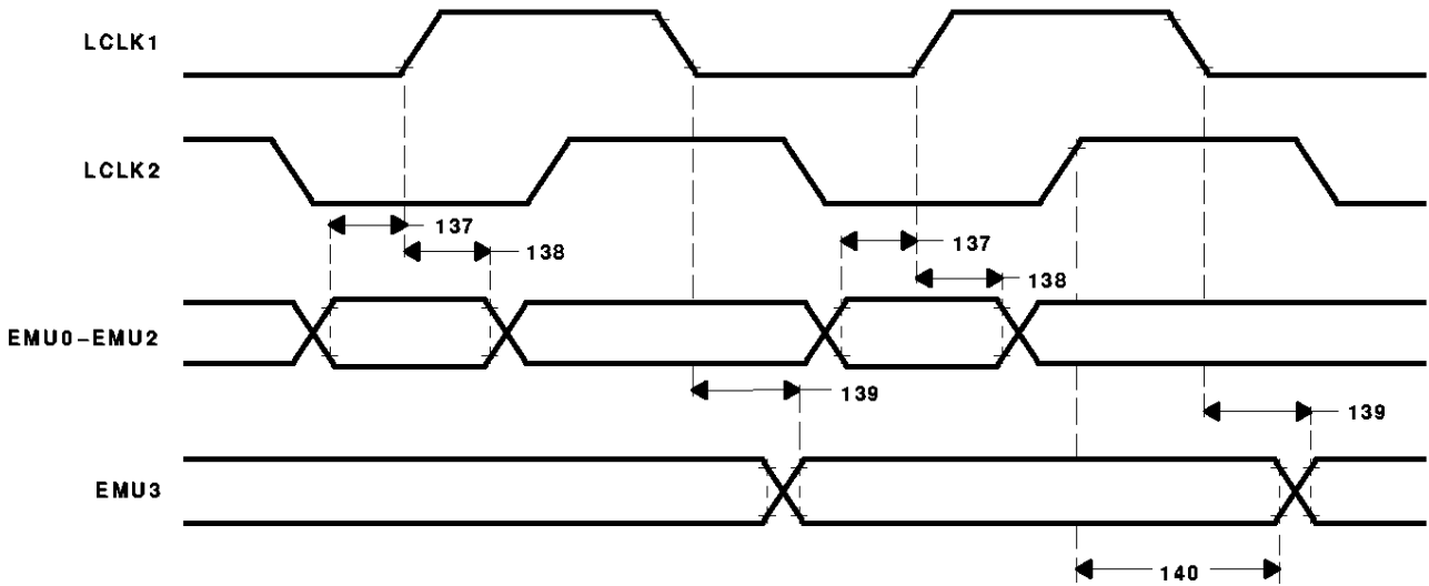
Figure 51. Emulator Interface Timing
