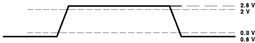
Figure 31. TTL-Level Outputs
