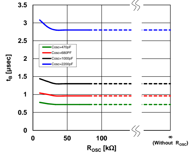
R_{OSC} , C_{OSC} vs. t_B V_{MM}=24V, T_a=25^\circ C
