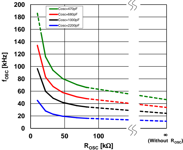
R_{OSC} , C_{OSC} vs. f_{OSC} V_{MM}=24V, T_a=25^\circ C
