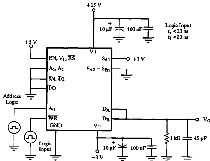
Figure 3. WR, Turn On Time
