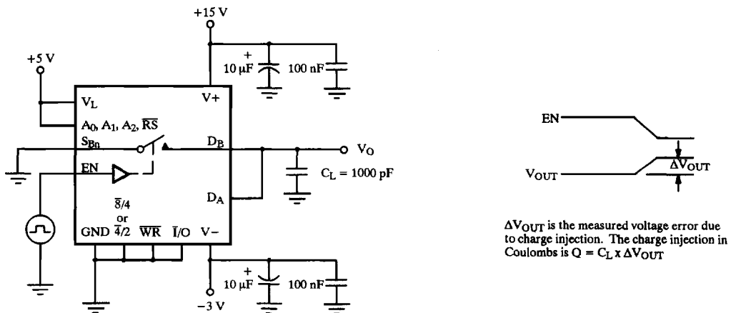
Figure 5. Charge Injection
