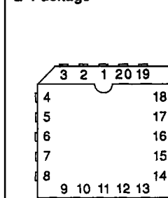
PLCC-20 (Top View) Q Package
