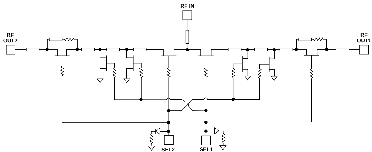
Figure 1. HMMC-2027 Schematic.
