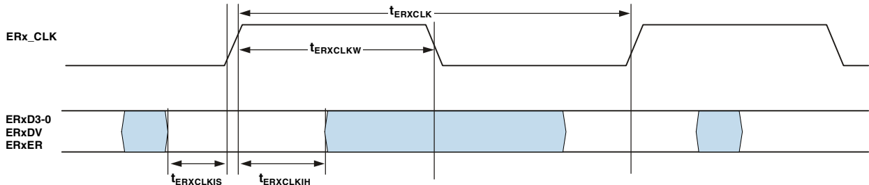
Figure 34. 10/100 Ethernet MAC Controller Timing: MII Receive Signal
