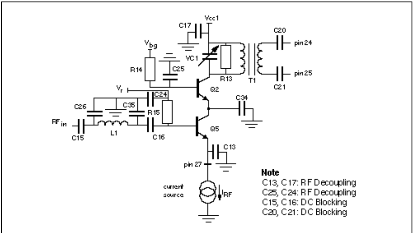
Fig.4 RF Amplifier
