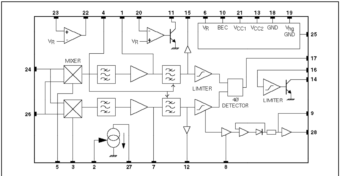
Fig.2 Block diagram of SL6609
