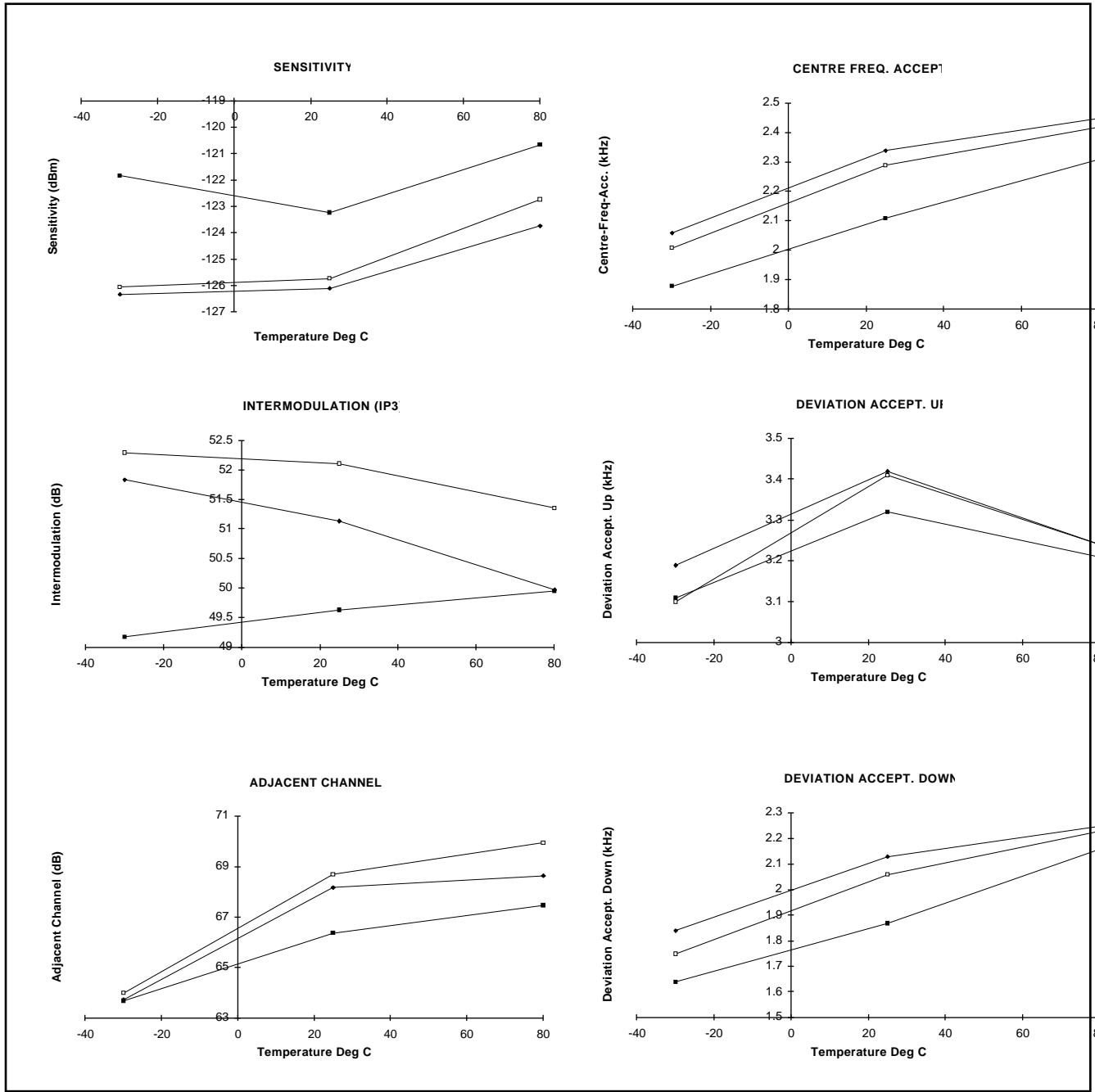
Fig.10 AC parameters vs. supply and temperature
