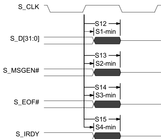
XpressFlow Bus Interface – Output float delay timing
