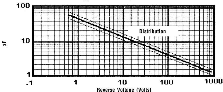
Typical Junction Capacitance
