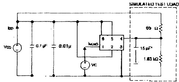
Figure 3. Output Test Conditions ( T_{amb} = 25 \pm 5^\circ \text{C} )
