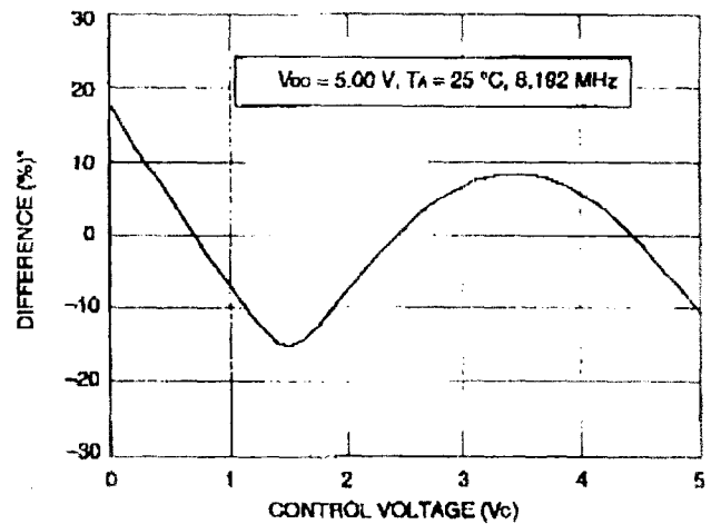
Figure 13. VCXO Linearity (Deviation From Best Linear Fit)
