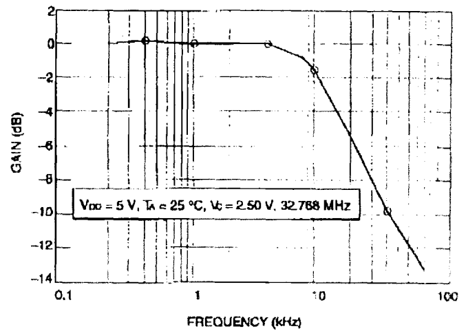
Figure 11. VCXO Input Frequency Response
