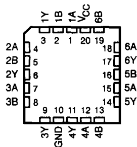
SN54ALS832A, SN54AS832B ... FK PACKAGE (TOP VIEW)
