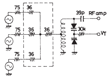
Intermodulation dummy
