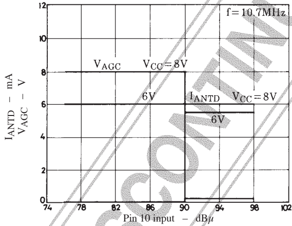
V AGC Input/Output Characteristic (AGC BLOCK)
