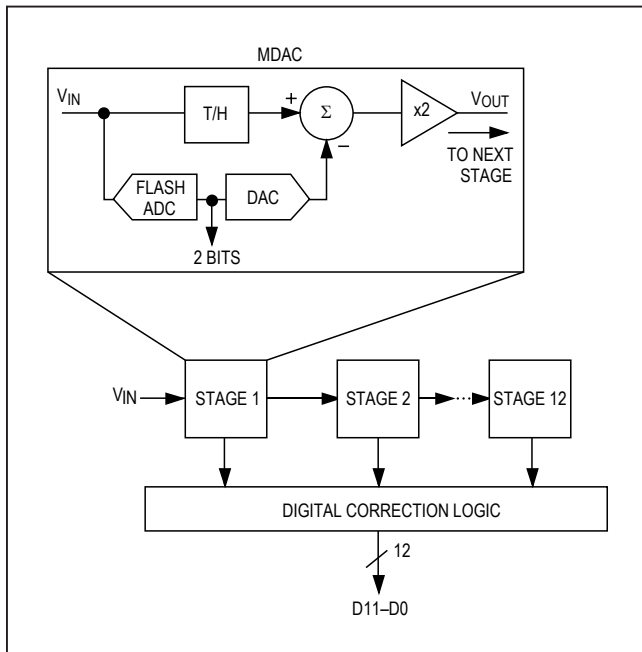
Figure 1. Pipelined Architecture
