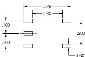
SUGGESTED FOOTPRINT
