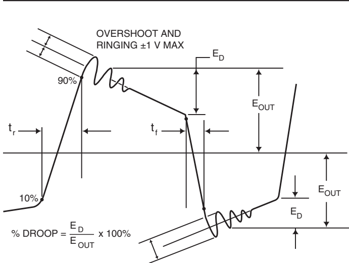
FIGURE 1. WAVEFORM INTEGRITY
