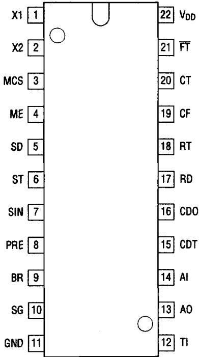
22-Pin Plastic DIP
