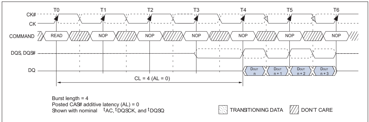
FIGURE 6 – CAS LATENCY (CL)
