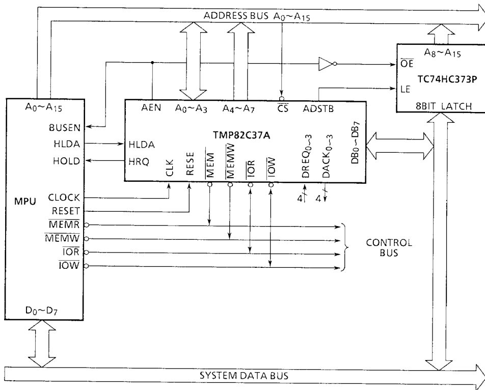
Figure 11.1 Basic System Connection Diagram
