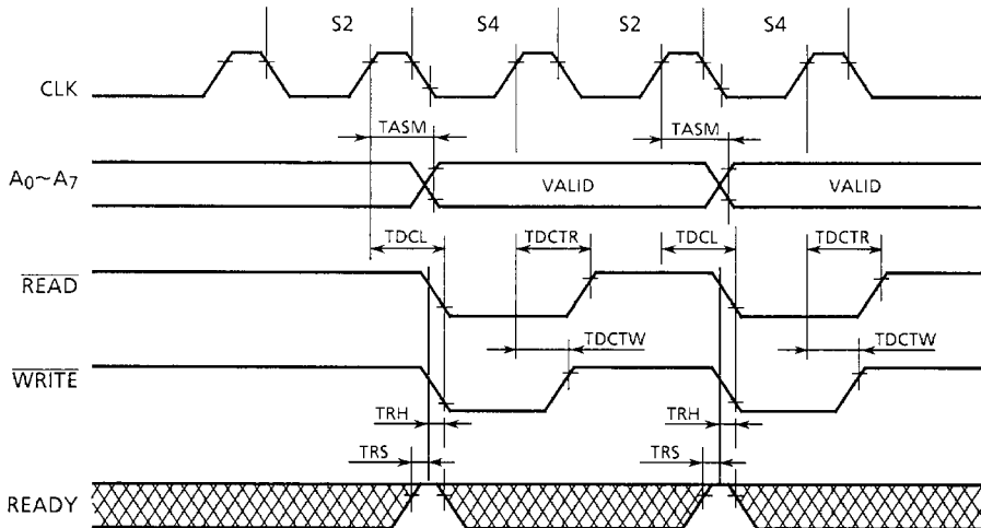
Timing Diagram 4 Memory-to-Memory Transfer
