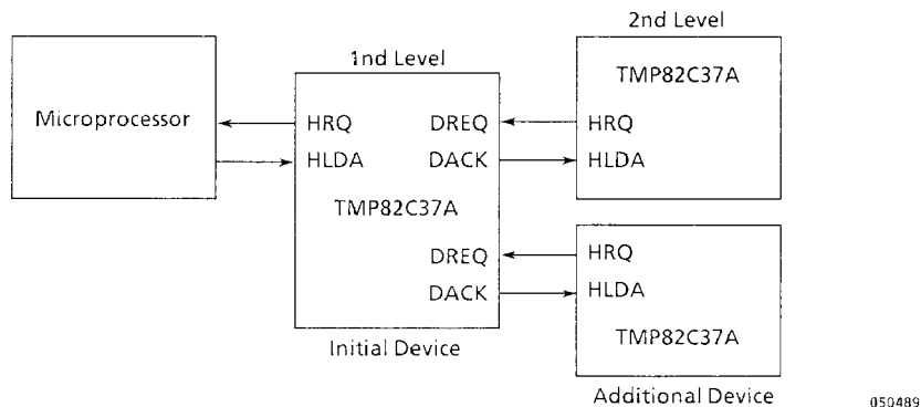
Figure 5.1 Example of Cascade Connection of TMP82C37A
