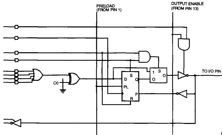
Figure 1. PLDC20RA10 Macrocell
