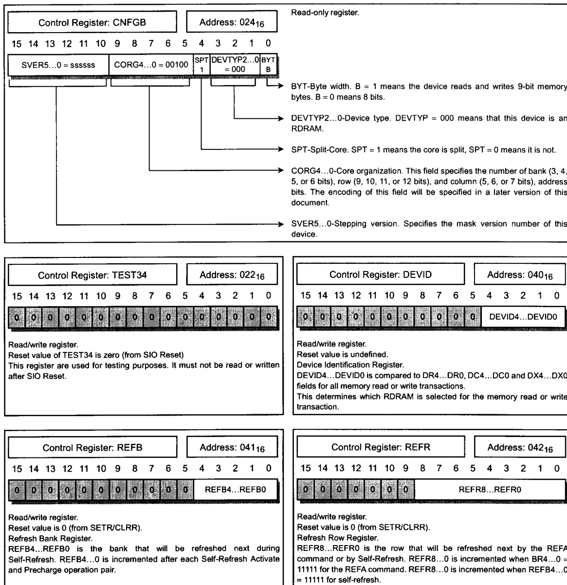
Figure 29. Control Registers
