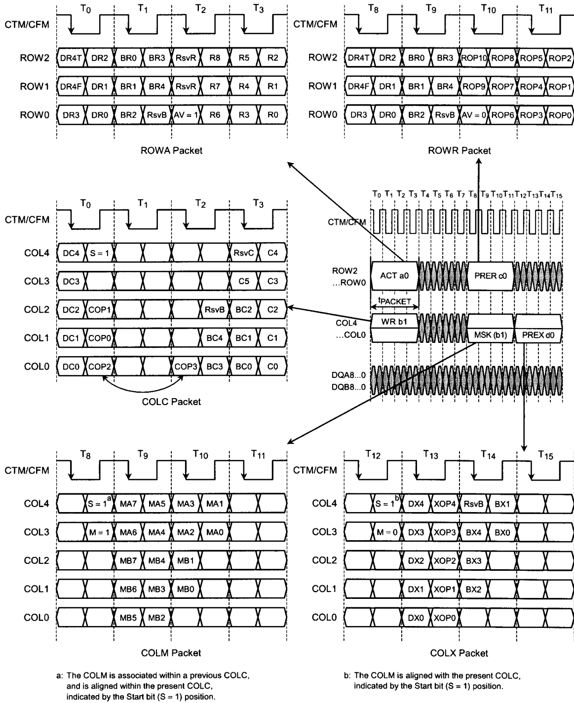
Figure 4. Packet Formats
