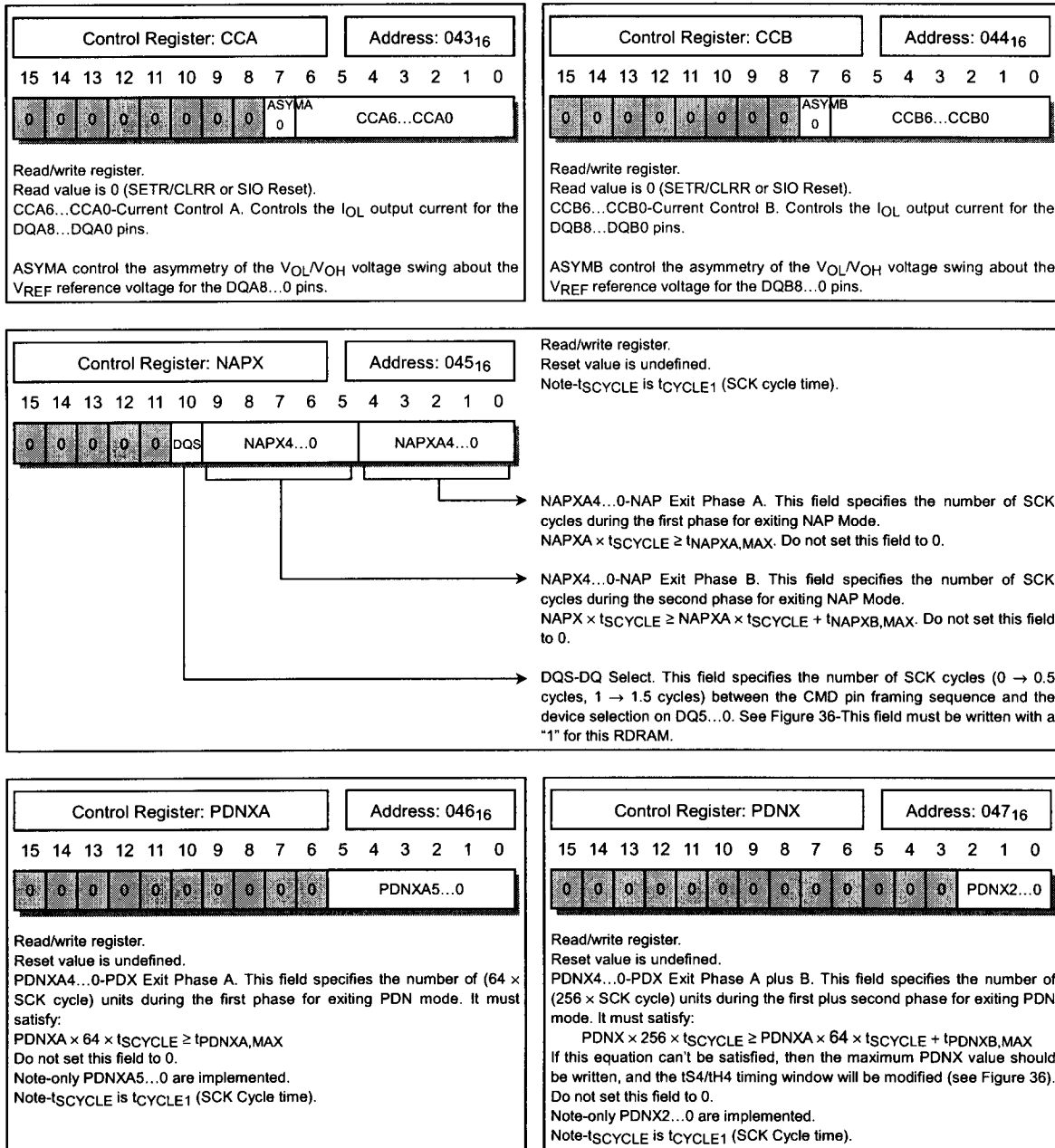
Figure 30. Control Registers
