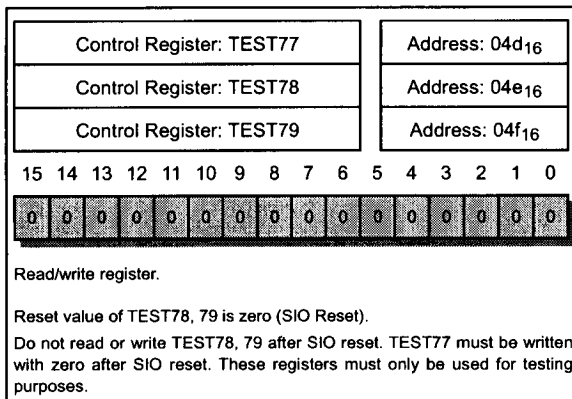
Figure 32. Control Registers
