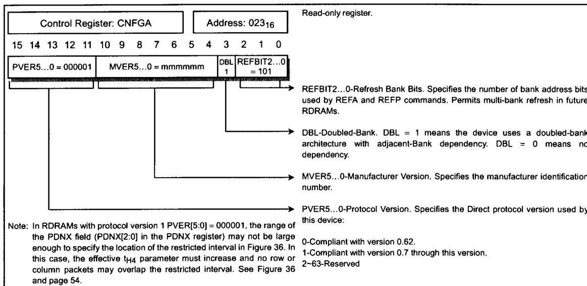
Figure 28. Control Registers
