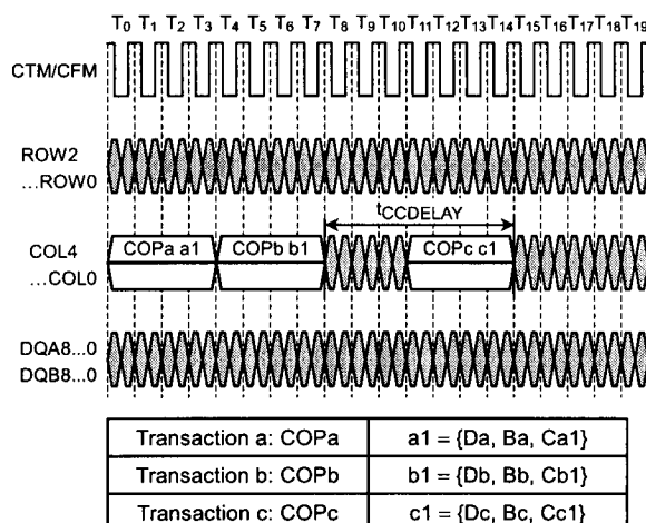
Figure 9. COL-to-COL Packet Interaction Timing
