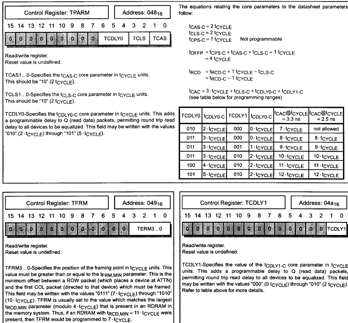
Figure 31. Control Registers
