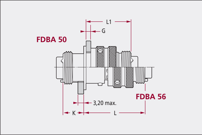
Square flange / Collettte carrée
