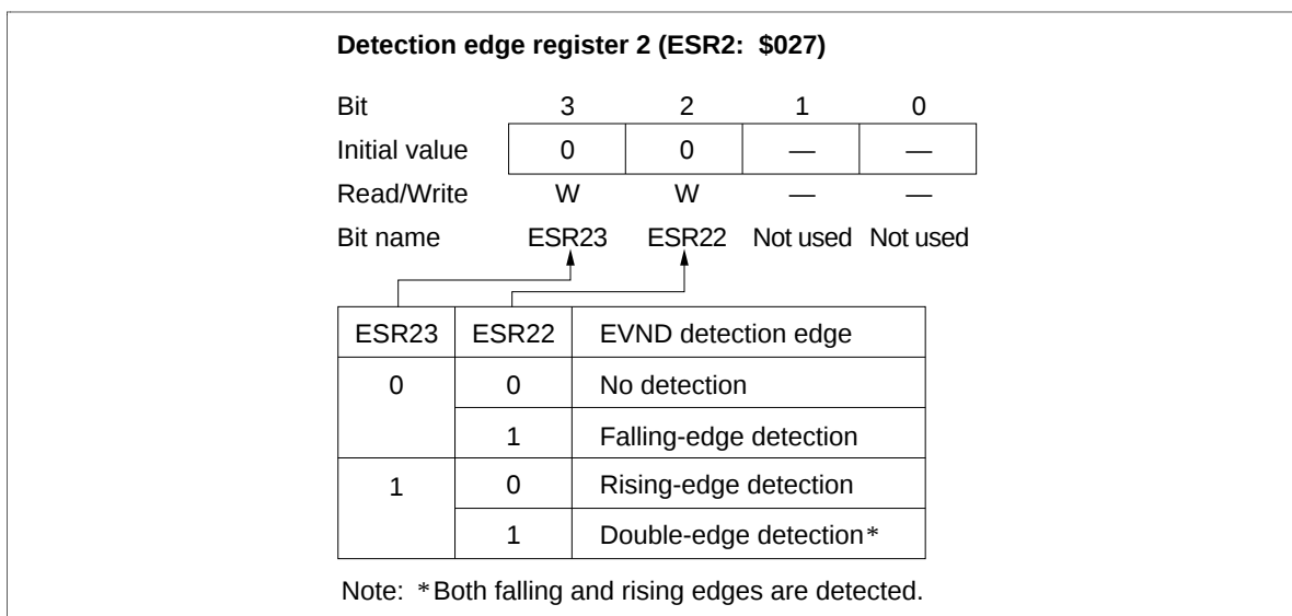
Figure 48 Detection Edge Select Register 2 (ESR2)
