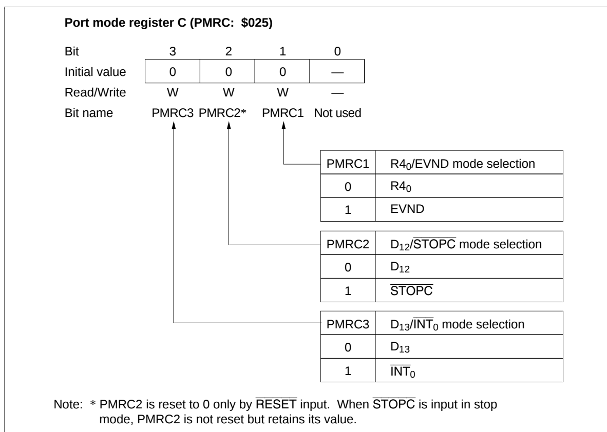
Figure 22 Port Mode Register C (PMRC)
