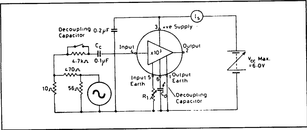
Fig.4 Gain Test Circuit (ZN459)
