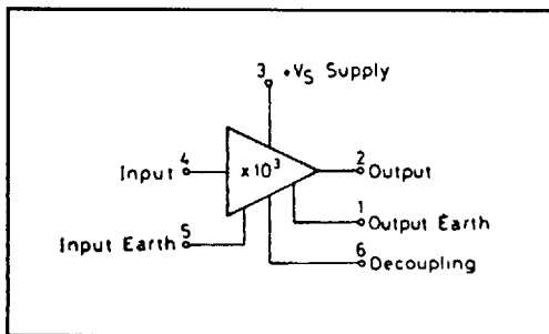
Fig.2 Pinning configuration - ZN459
