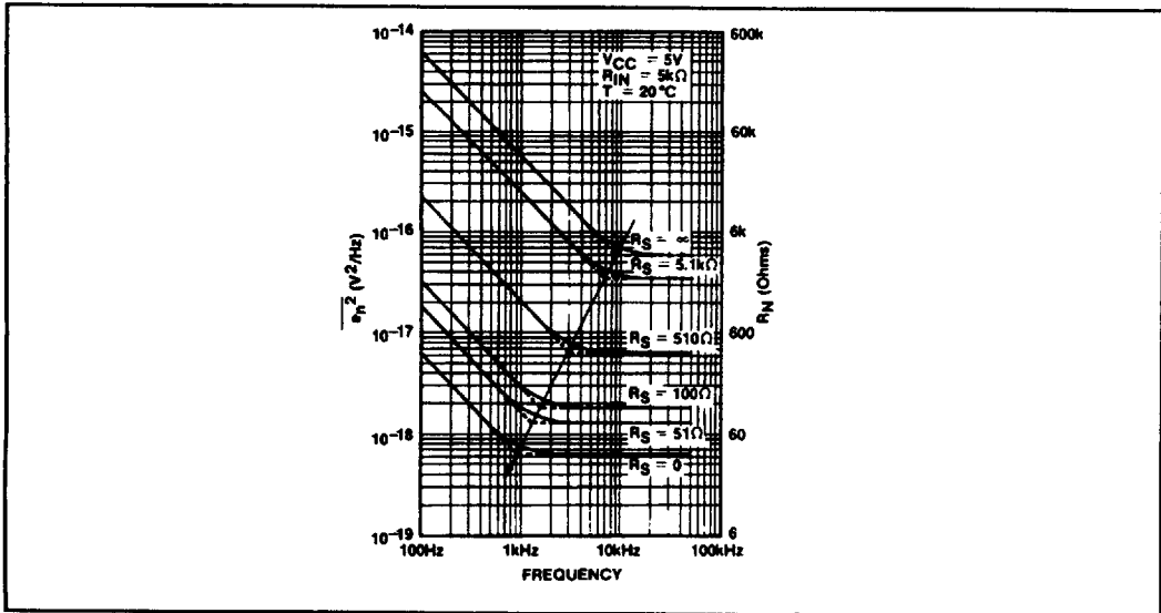
Fig.13 Noise Voltage
