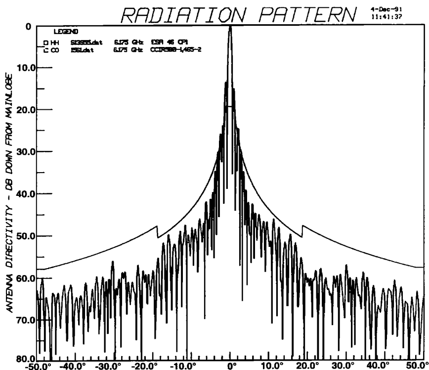
ES46-CCP2, 6.175 GHz, LHCP, \pm 50^\circ Azimuth
