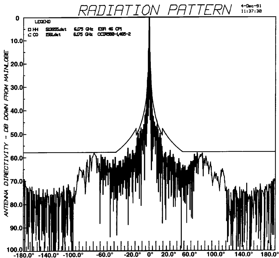
ES46-CCP2, 6.175 GHz, LHCP, \pm 180^\circ Azimuth
