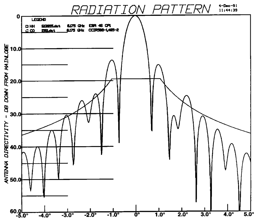
ES46-CCP2, 6.175 GHz, LHCP, \pm 5^\circ Azimuth
