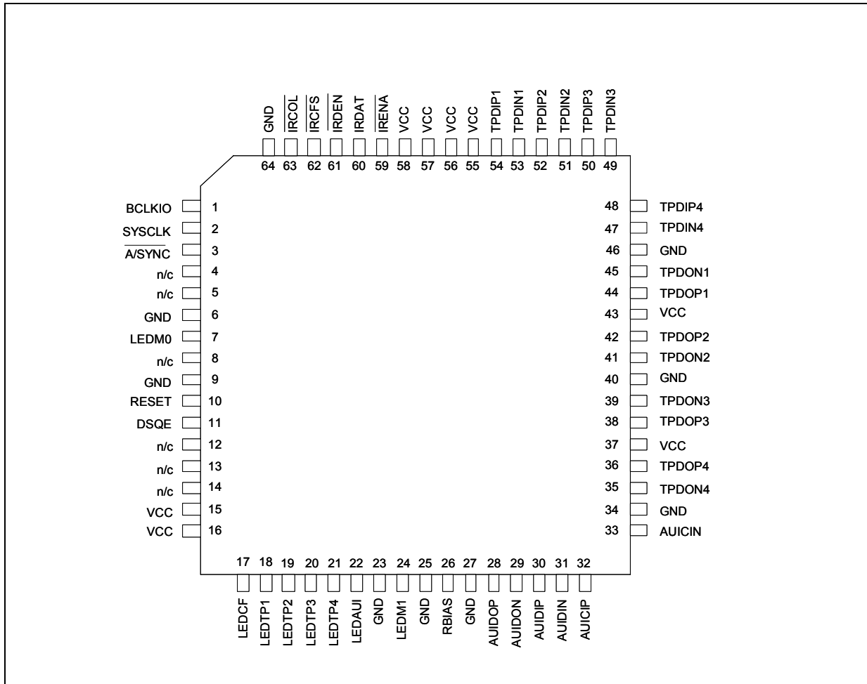
Figure 2 LXT915 Repeater Pin Assignments
