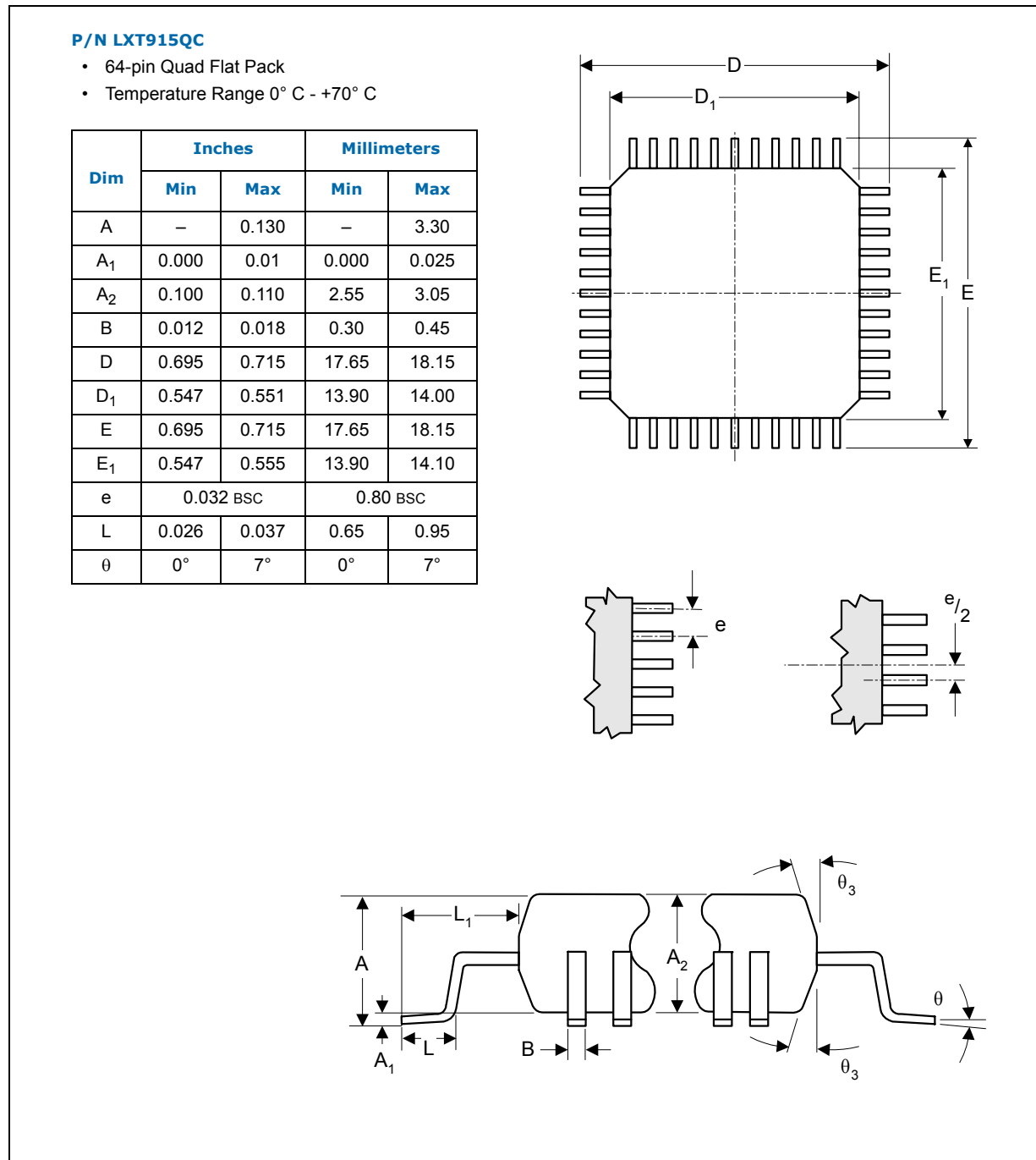
Figure 9 Package Specifications
