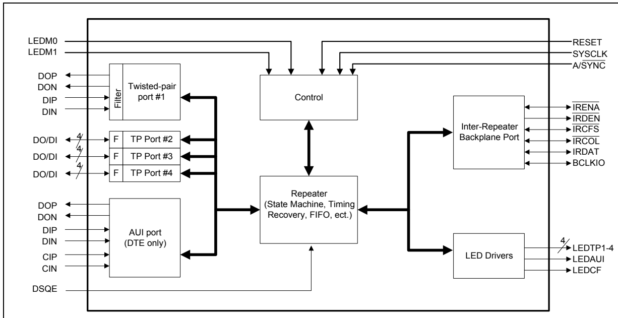
Figure 1 LXT915 Repeater Block Diagram
