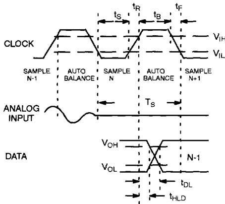
Figure 1. MP8798 Timing Diagram
