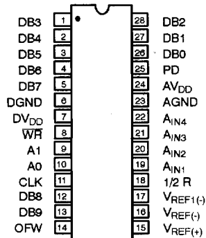
28 Pin PDIP (0.300")
