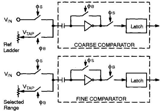
Figure 2. MP8798 Comparators
