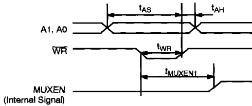
Figure 11. Analog MUX Timing
