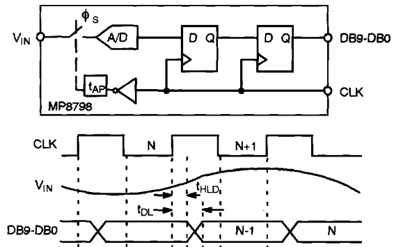
Figure 12. MP8798 Functional Equivalent Circuit and Interface Timing
