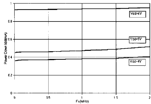
Graph 4. Power Down Current vs. Sampling Frequency
