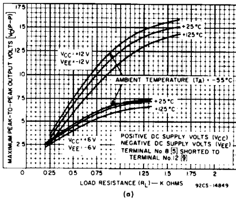
Fig. 9 — Maximum peak-to-peak output voltage vs. load resistance for CA3010A, CA3015A
