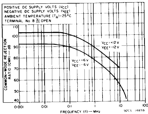
Fig. 12 — Common-mode rejection ratio vs. frequency.
