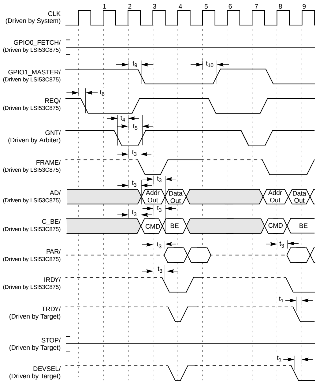
Figure 7.20 Burst Write
