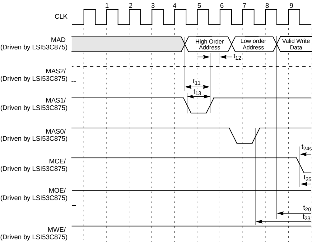
Figure 7.30 Write Cycle, Slow Memory ( \leq 64 Kbyte)
