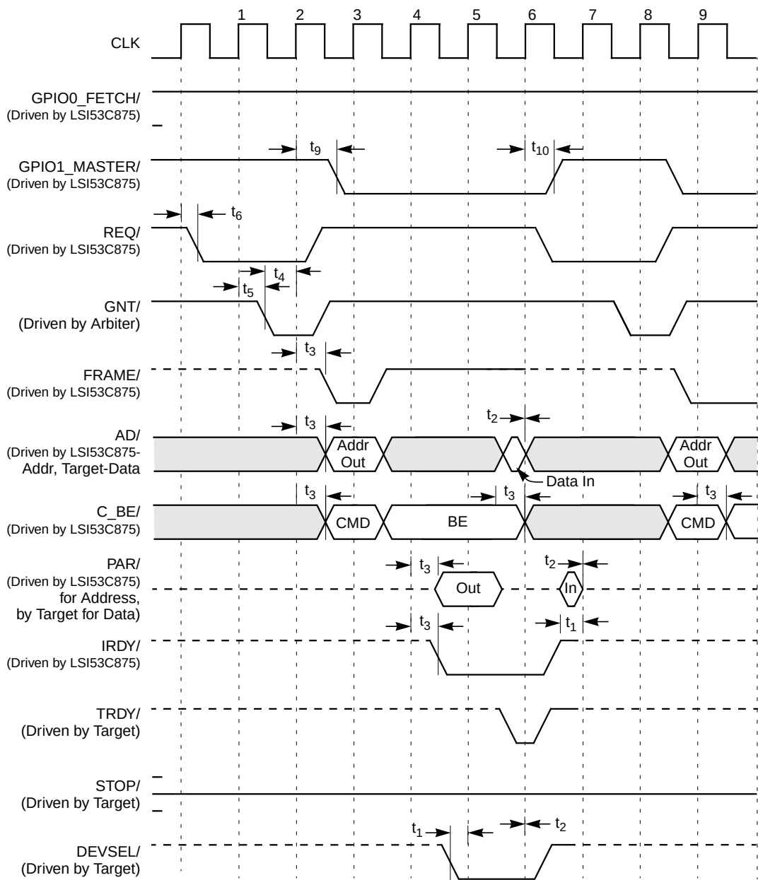
Figure 7.19 Burst Read
