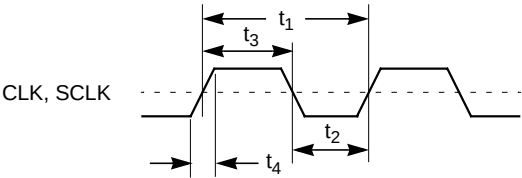
Figure 7.6 Clock Waveforms
