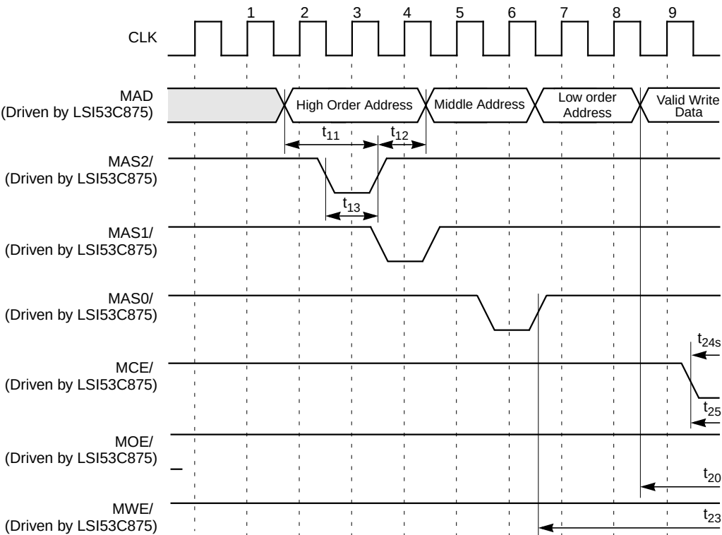
Figure 7.26 Write Cycle, Slow Memory ( \geq 64 Kbyte)
