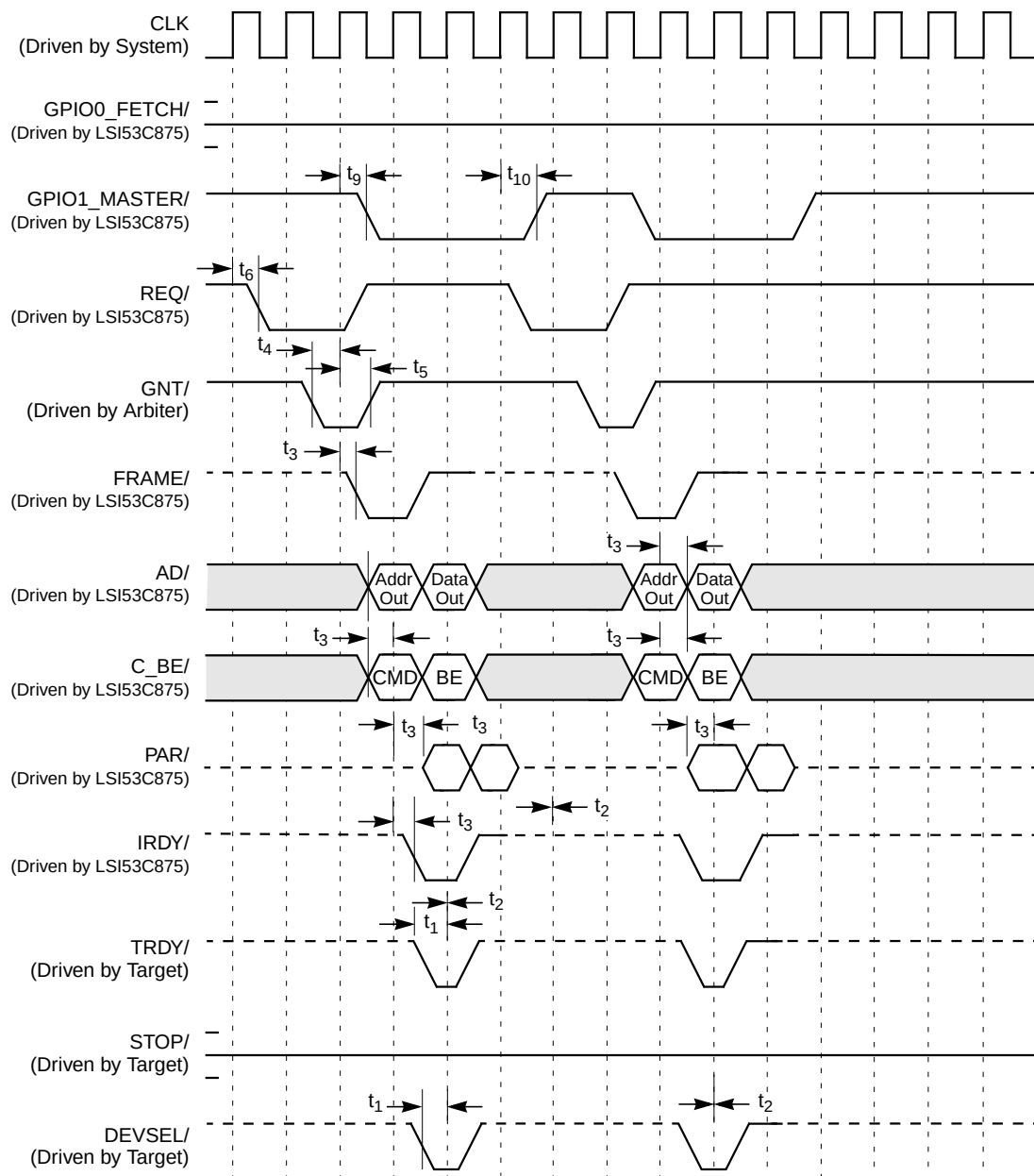
Figure 7.18 Back-to-Back Write
