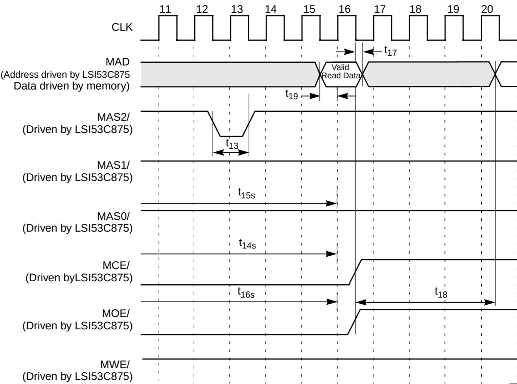
Figure 7.25 Read Cycle, Slow Memory ( \geq 64 Kbyte) (Cont.)
