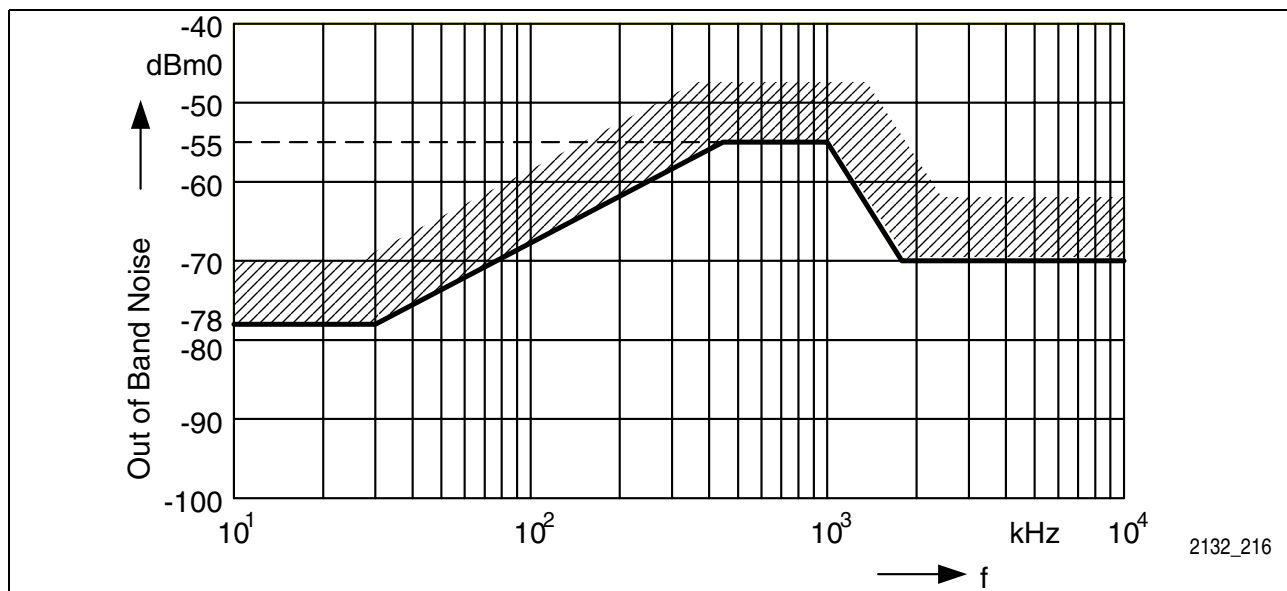
Figure 13 Analog Output: Out-of-Band Idle Channel Noise
