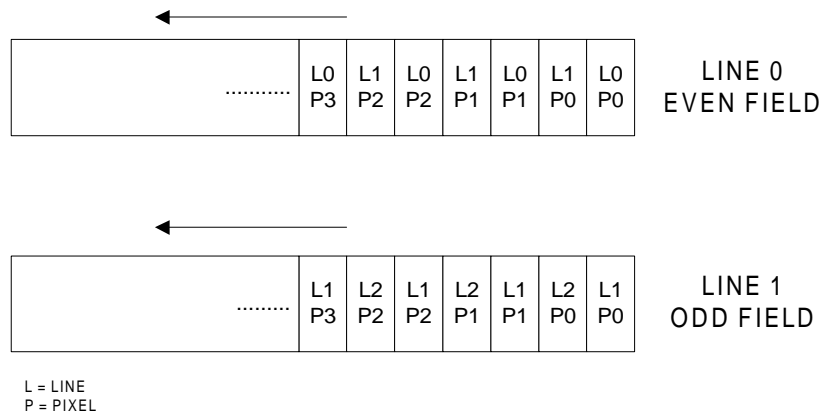
DATA PIPELINE AFTER MMUX, 2X CLOCKING
