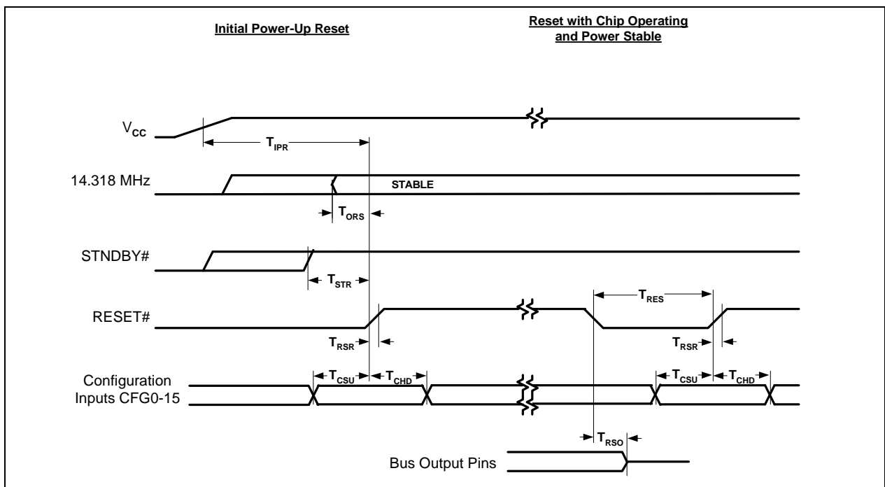
Figure 3-3: Reset Timing
