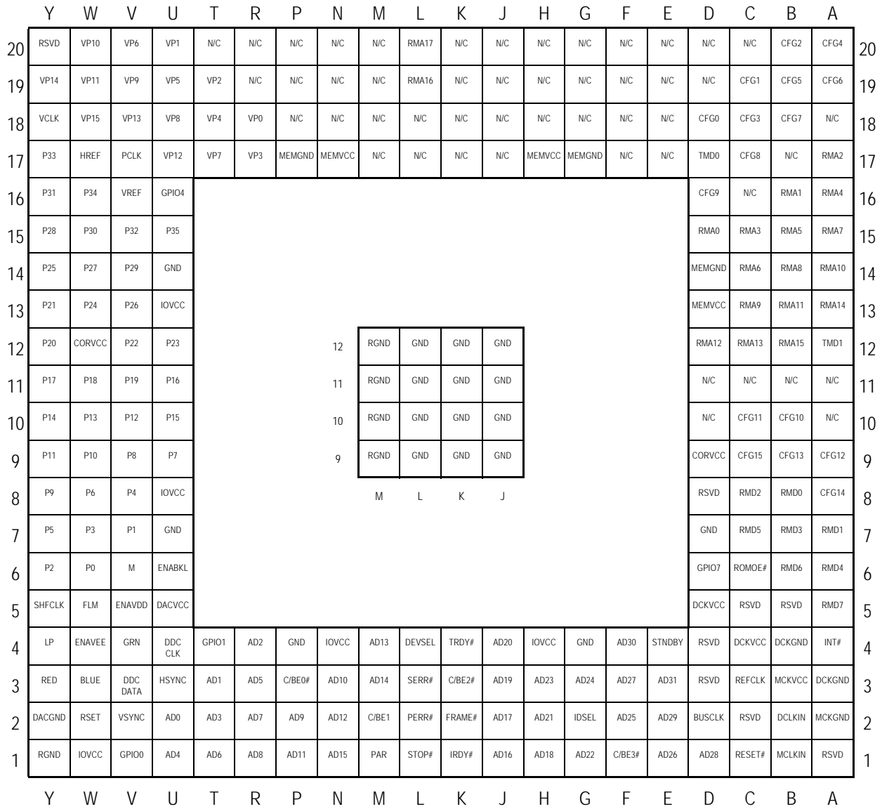
Figure 2-2: Pin Diagram
