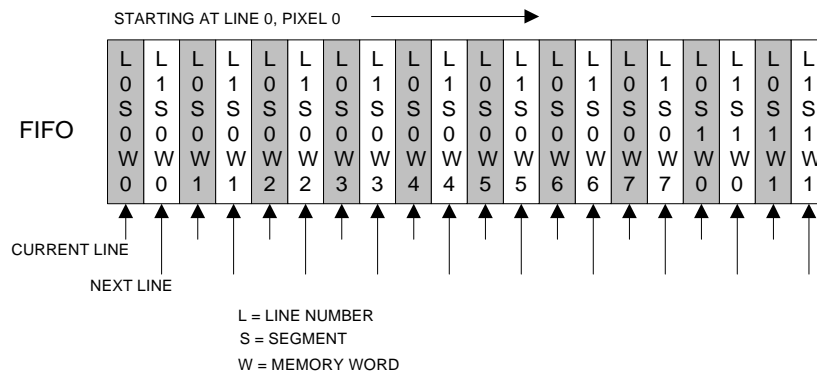
FIFO CONTENTS IN FLICKER REDUCTION MODE
