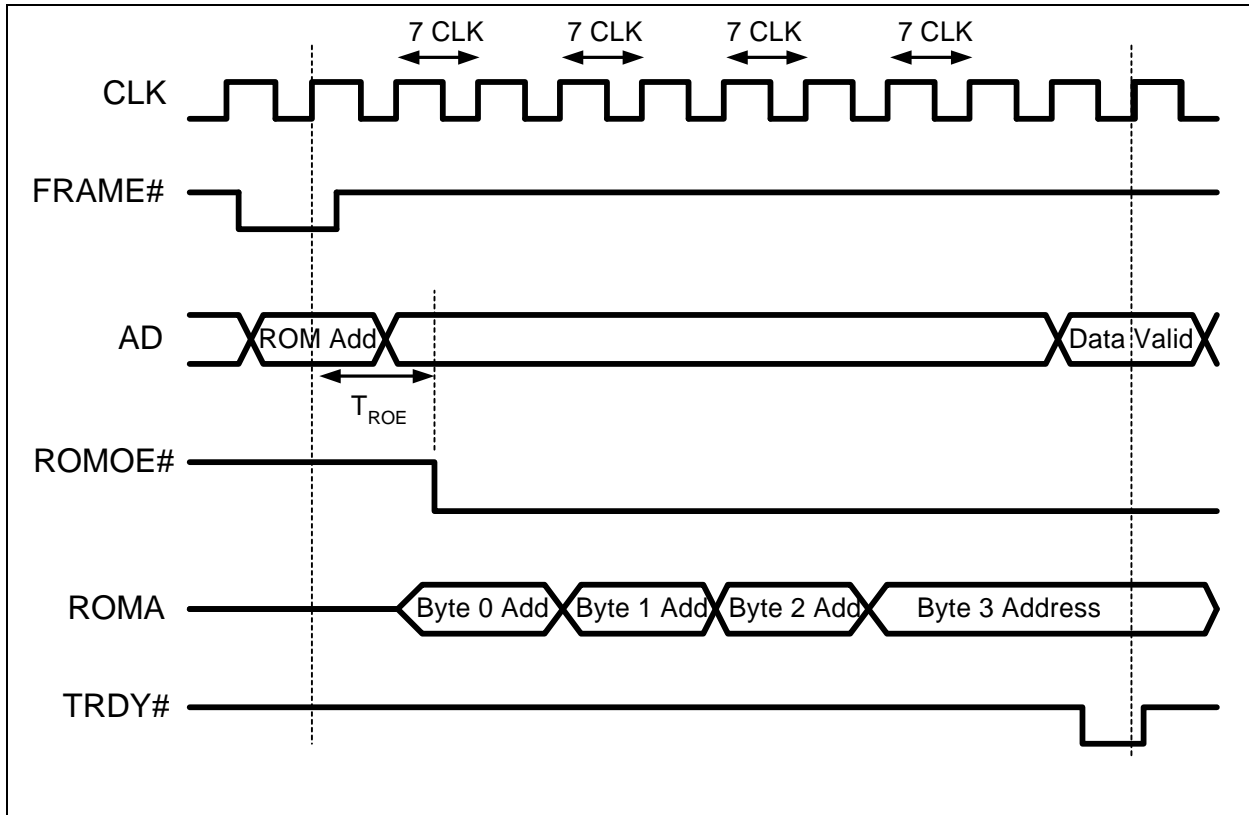
Figure 3-6: PCI BIOS ROM Timing
