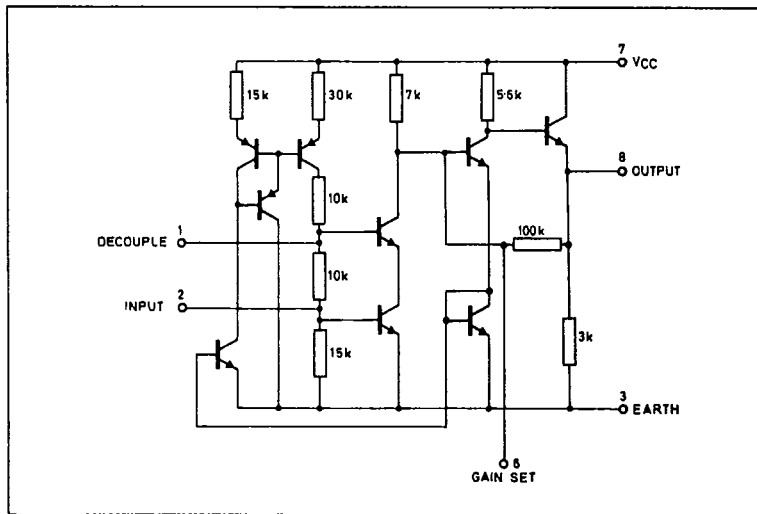
Fig.8 Circuit diagram
