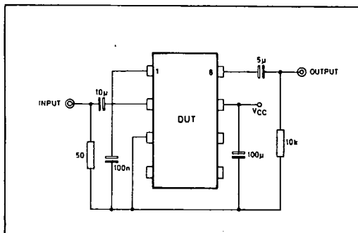
Fig.3 Test circuit
