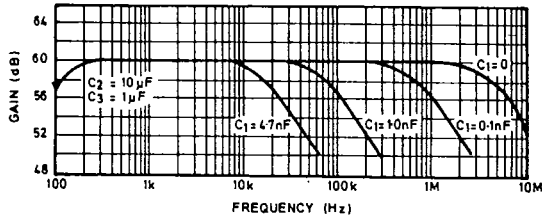
Fig.5 Gain v. frequency
