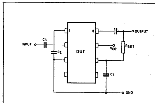
Fig.4 Typical application
