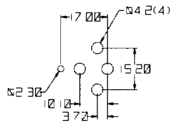
RECOMMENDED PCB LAYOUT (BOTTOM VIEW)
