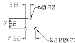
RECOMMENDED PCB LAYOUT (BOTTOM VIEW)
