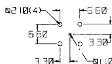
RECOMMENDED PCB LAYOUT (BOTTOM VIEW)
