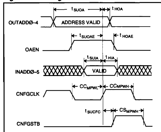
Figure 4. Reconfiguration Mode
