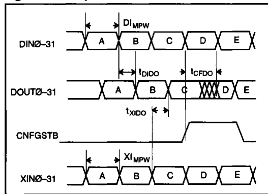
Figure 3. Transparent Mode
