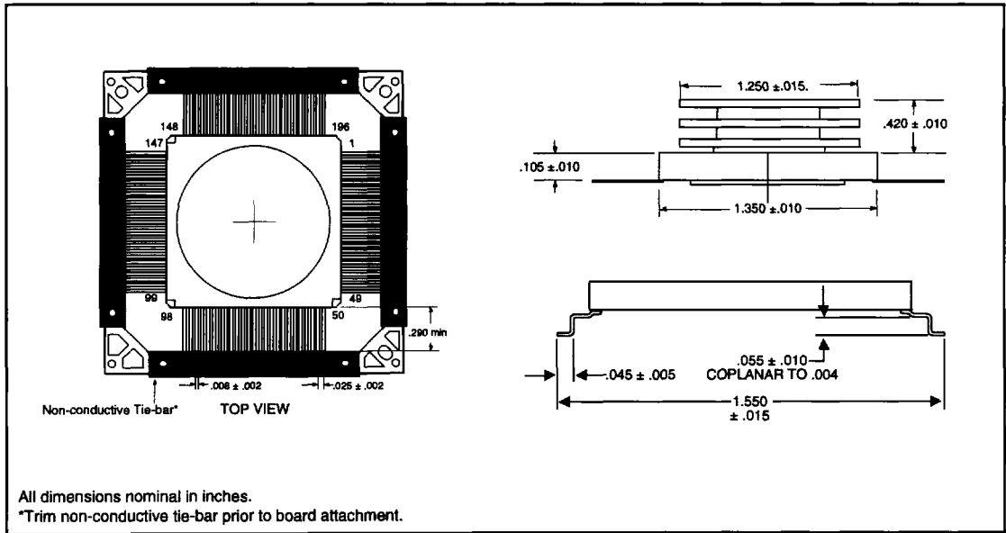
Figure 5.196 LDCC Package
