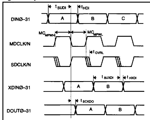
Figure 2. Synchronous Mode
