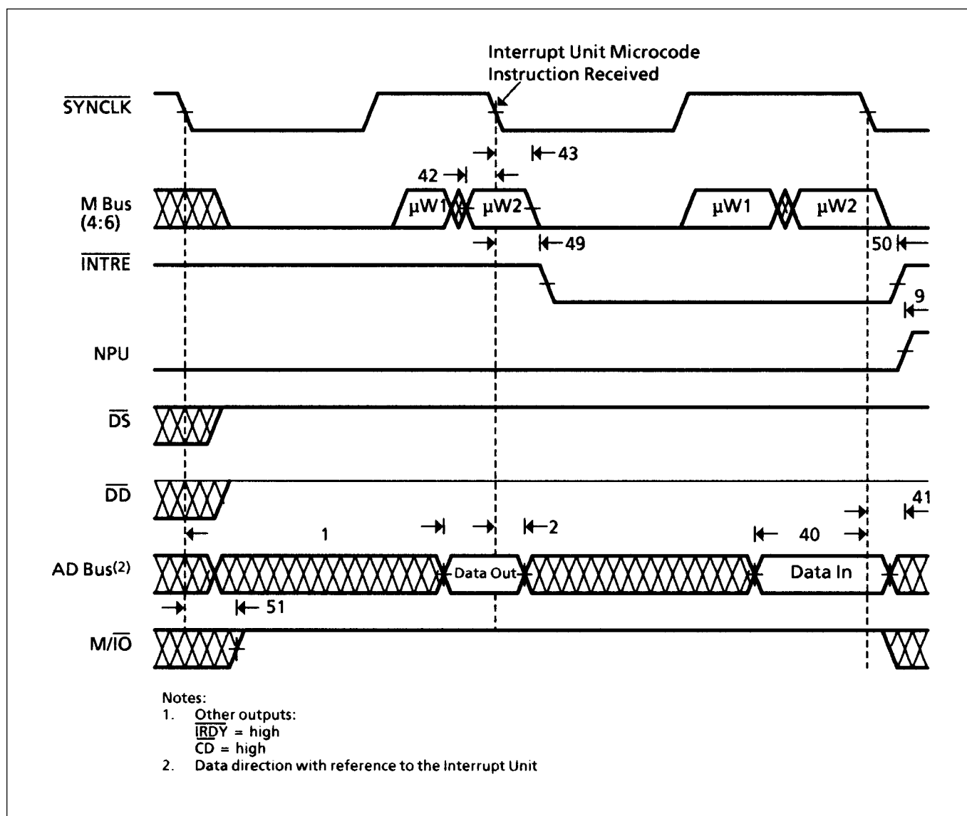
Figure 4: Microcode Operations
