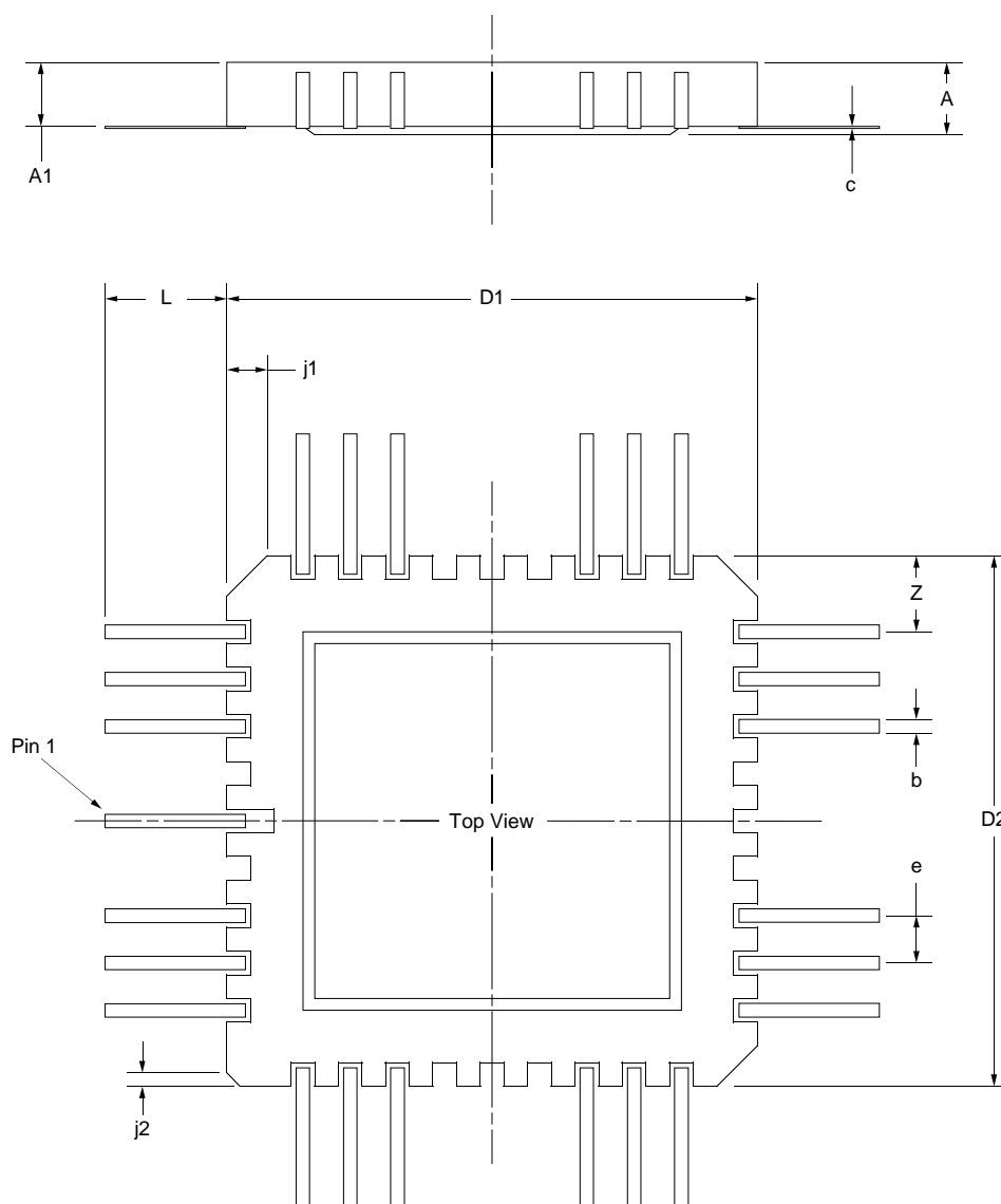
Figure 18a: 68-Lead Topbrazed Flatpack - Package Style F
