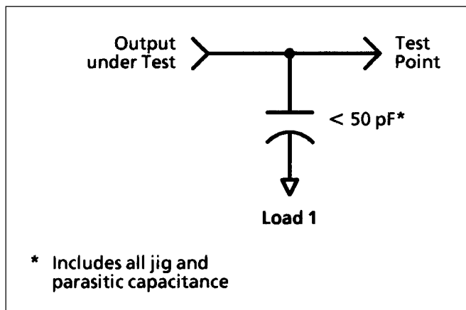
Figure 3: Test Load
