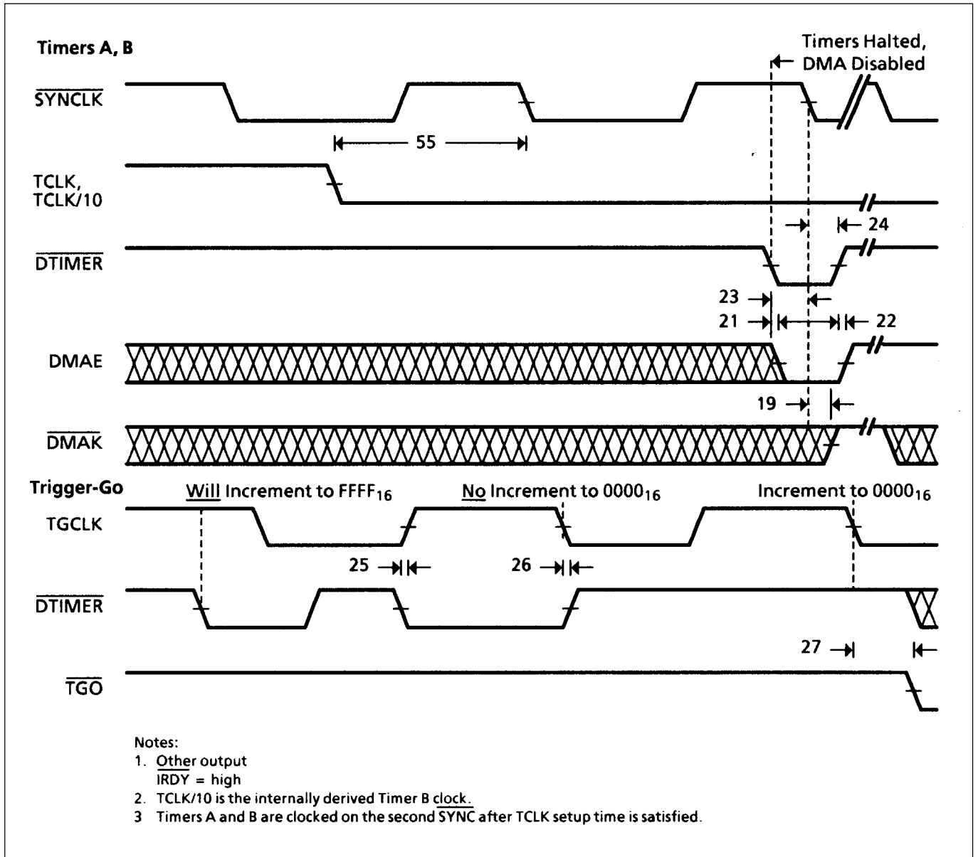
Figure 15: Timer Operations
