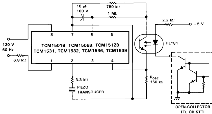
FIGURE 7. NONTELEPHONE APPLICATION
