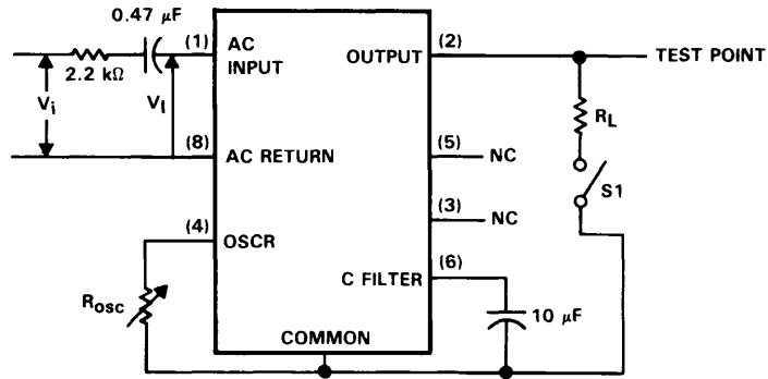
FIGURE 1. TEST CIRCUIT
