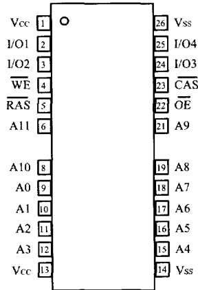
24(26)TSOP II
