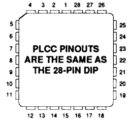
28-Pin PLCC
