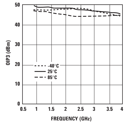
Figure 40. OIP3 vs. Temperature and Frequency at optimum OIP3.
