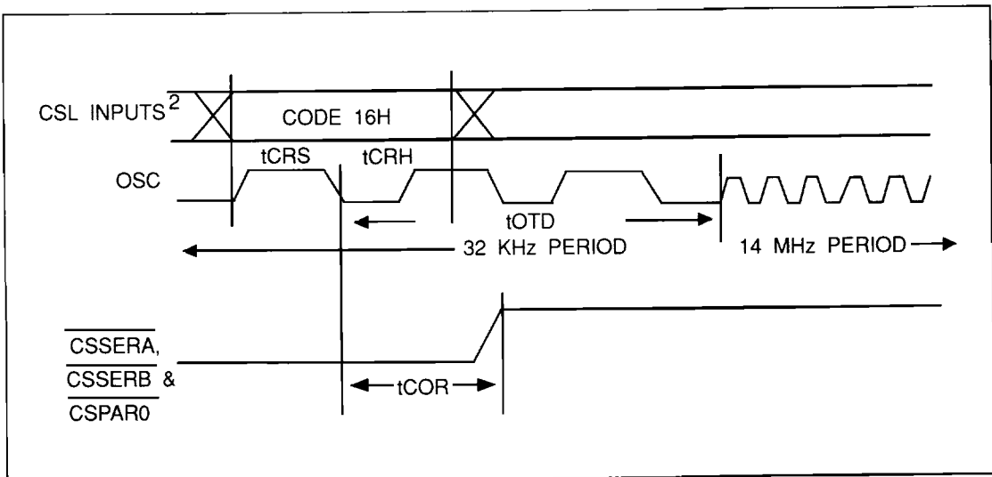
FIGURE 4-20. SUSPEND TO RESUME SUPPORT LOGIC
