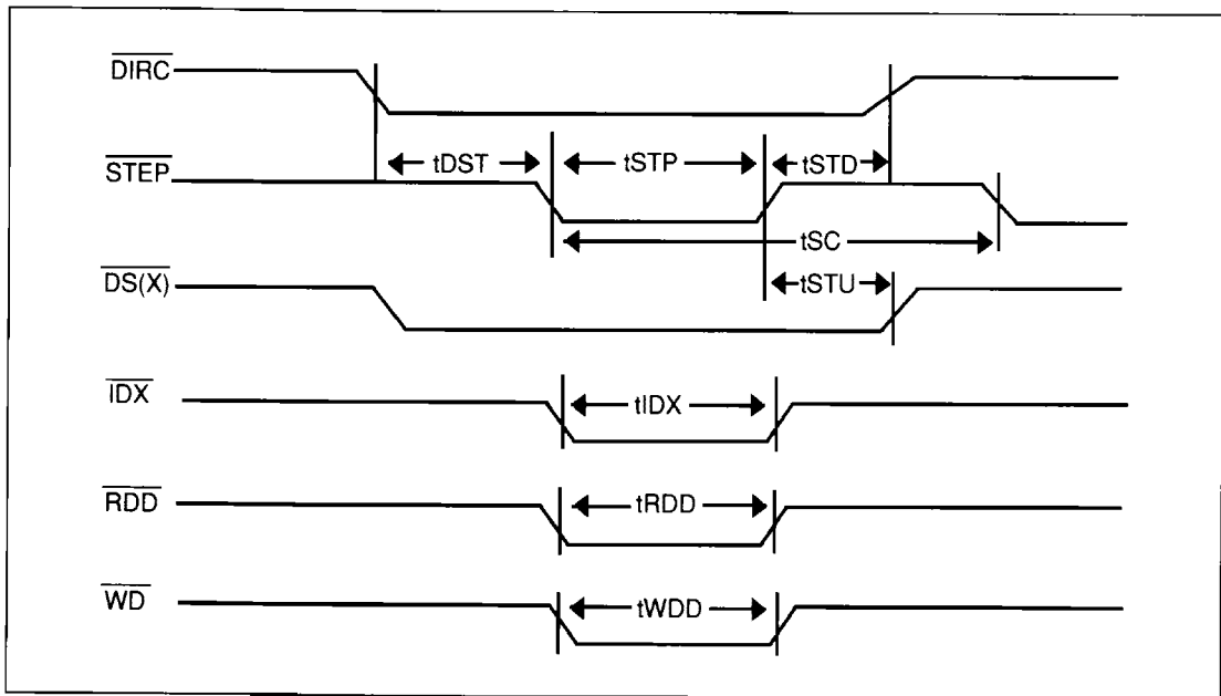
FIGURE 4-8. FDC DISK DRIVE TIMING DIAGRAM
