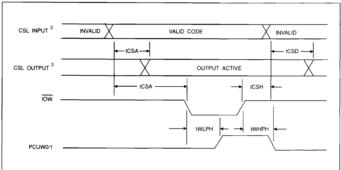
FIGURE 4-21. CHIP SELECT LOGIC DECODE TIMING DIAGRAM
