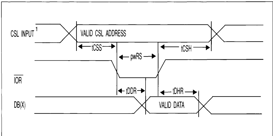
FIGURE 4-9. RTC AND RAM READ TIMING DIAGRAM
