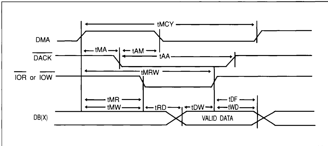
FIGURE 4-5. FDC DMA TIMING DIAGRAM
