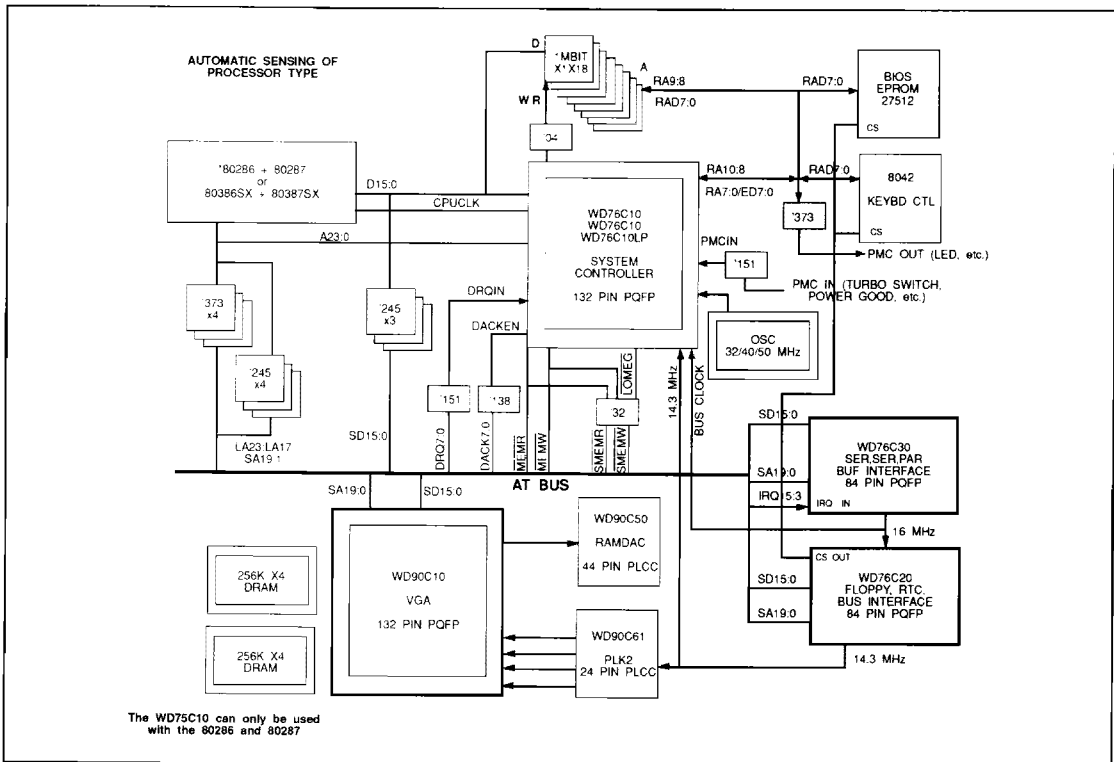
FIGURE 2-1. SYSTEM LEVEL FUNCTIONAL BLOCK DIAGRAM
